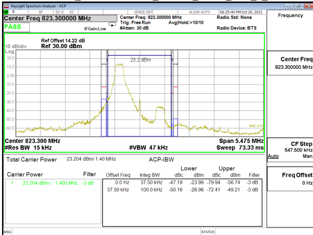
Emission Mask_Band26-Part90s_1.4MHz_QPSK_RB1_0_CH26783
