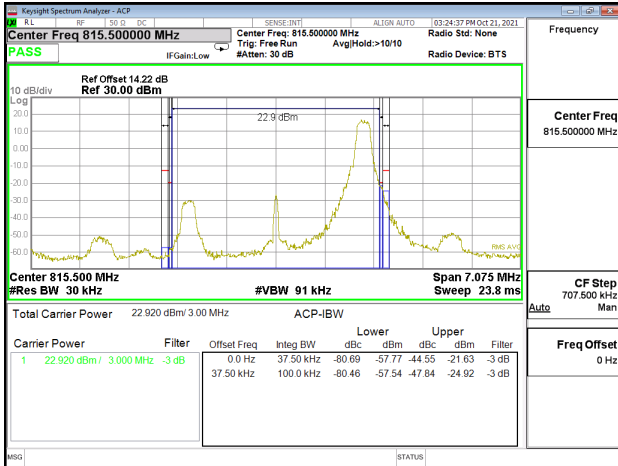
Emission Mask_Band26-Part90s_3MHz_QPSK_RB1_14_CH26740
