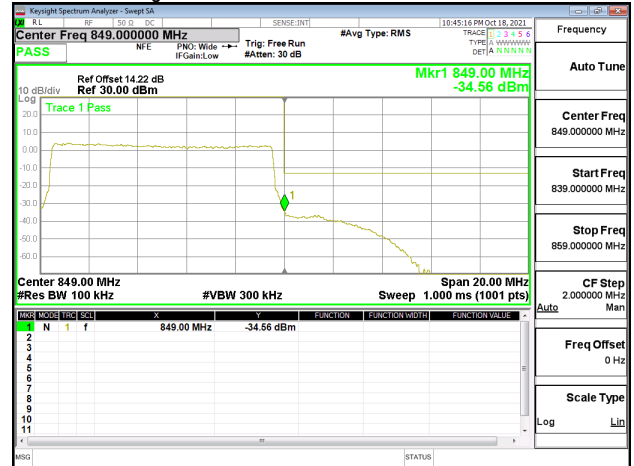
Band Edge_Band26_15MHz_QPSK_RB1_0_CH26865
