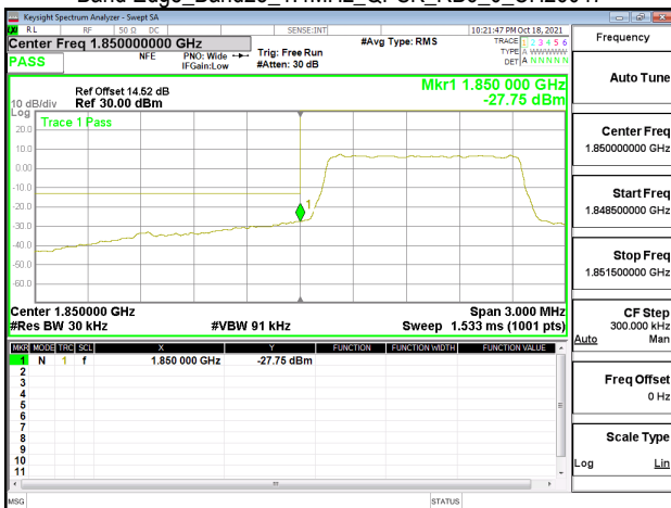
Band Edge_Band25_1.4MHz_QPSK_RB6_0_CH26047
