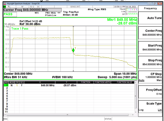
Band Edge_Band26_5MHz_QPSK_RB25_0_CH27015
