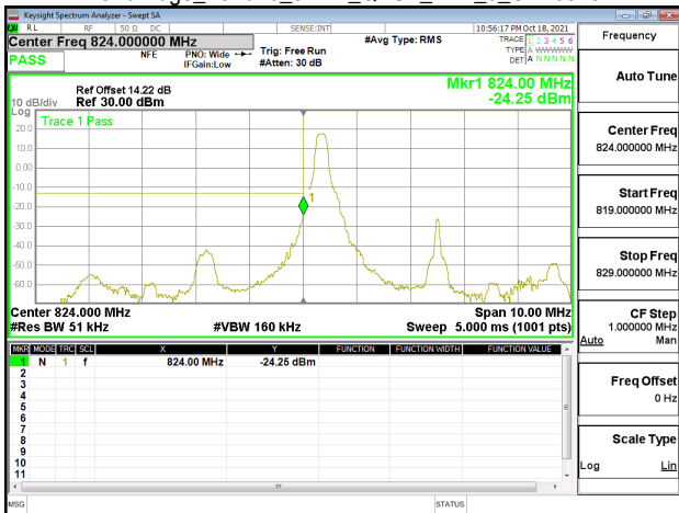
Band Edge_Band26_5MHz_QPSK_RB1_0_CH26815
