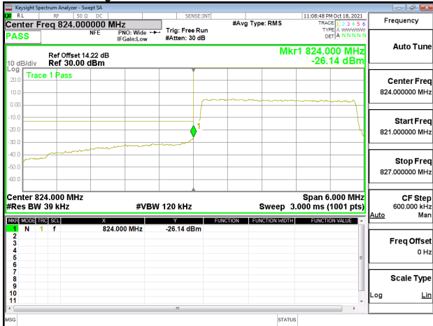
Band Edge_Band26_3MHz_QPSK_RB15_0_CH27025
