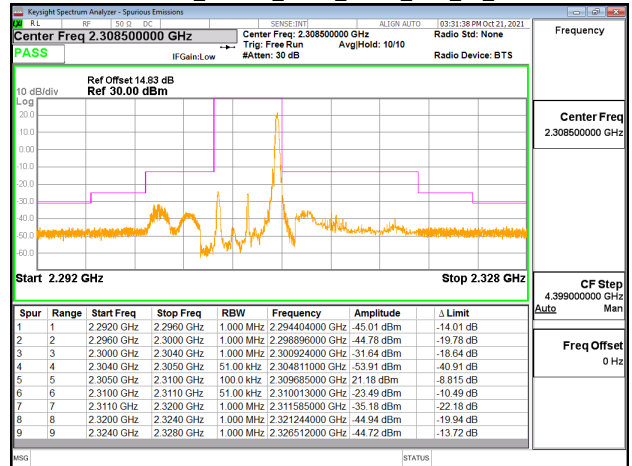
Emission Mask_Band30_5MHz_QPSK_RB1_24_CH27685
