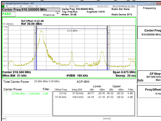
Emission Mask_Band26-Part90s_5MHz_QPSK_RB1_0_CH26740
