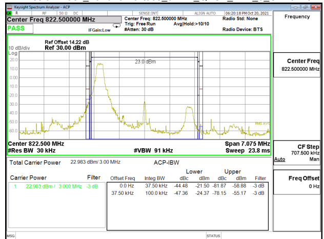
Emission Mask_Band26-Part90s_3MHz_QPSK_RB1_0_CH26775
