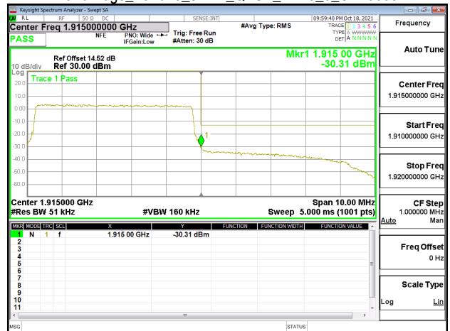
Band Edge_Band25_5MHz_QPSK_RB25_0_CH26665
