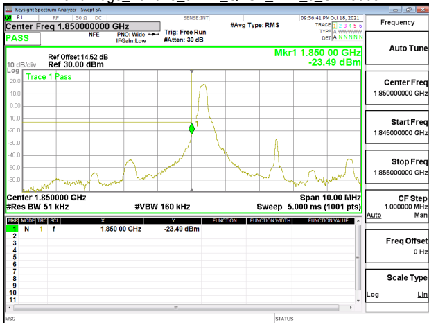
Band Edge_Band25_5MHz_QPSK_RB1_0_CH26065
