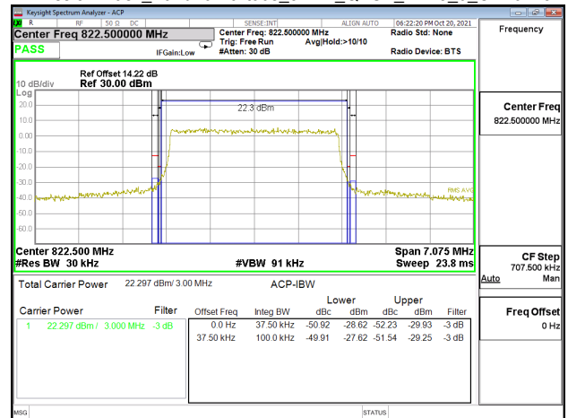
Emission Mask_Band26-Part90s_3MHz_QPSK_RB15_0_CH26775
