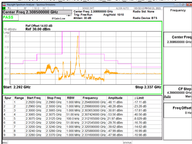
Emission Mask_Band30_5MHz_QPSK_RB1_24_CH27735
