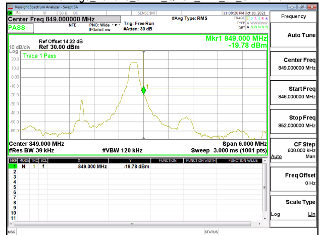
Band Edge_Band26_3MHz_QPSK_RB1_14_CH27025
