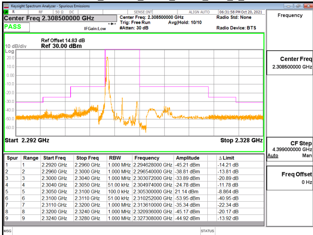
Emission Mask_Band30_5MHz_QPSK_RB1_0_CH27685
