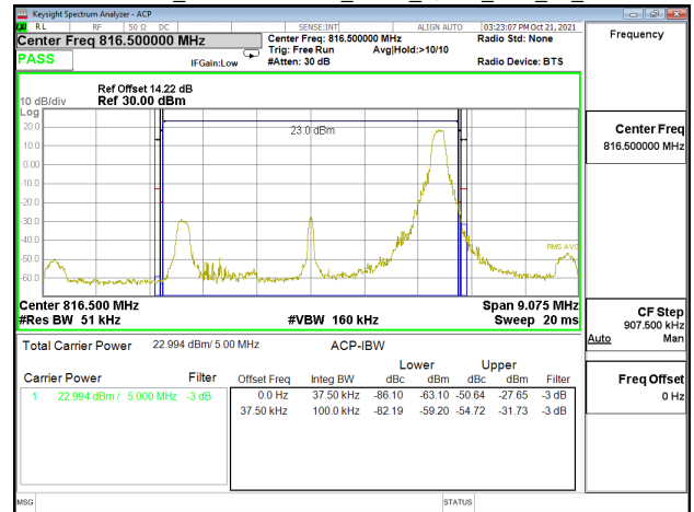
Emission Mask_Band26-Part90s_5MHz_QPSK_RB1_24_CH26740
