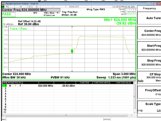
Band Edge_Band26_1.4MHz_QPSK_RB6_0_CH26797
