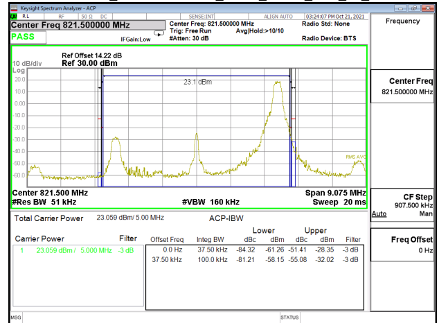
Emission Mask_Band26-Part90s_5MHz_QPSK_RB1_24_CH26765
