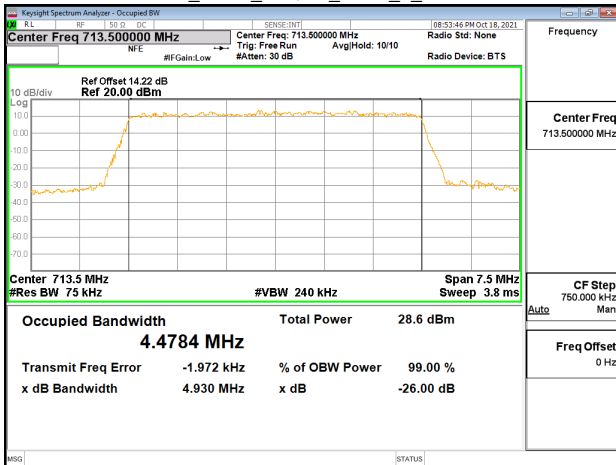
Band17_5MHz_64QAM_RB25_0_CH23825
