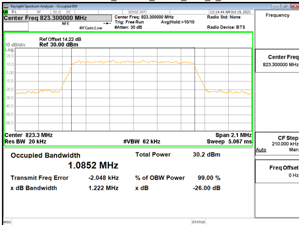
Band26-Part90s_1.4MHz_QPSK_RB6_0_CH26783
