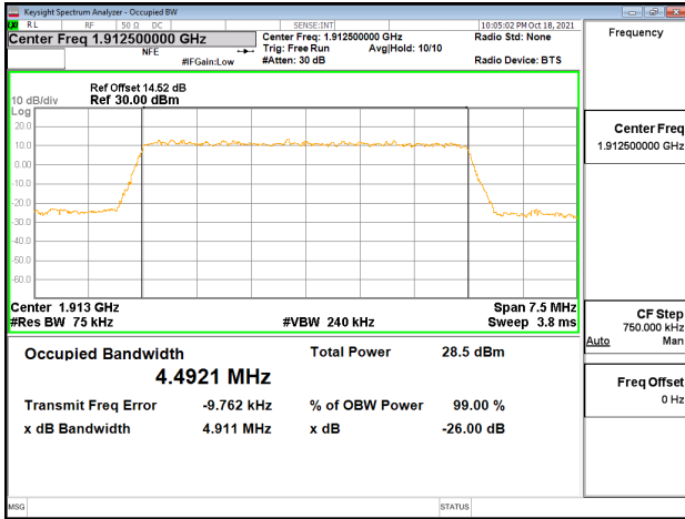
Band25_5MHz_64QAM_RB25_0_CH26665
