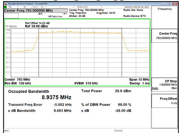
Band14_10MHz_64QAM_RB50_0_CH23330
