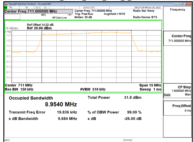
Band17_10MHz_QPSK_RB50_0_CH23800
