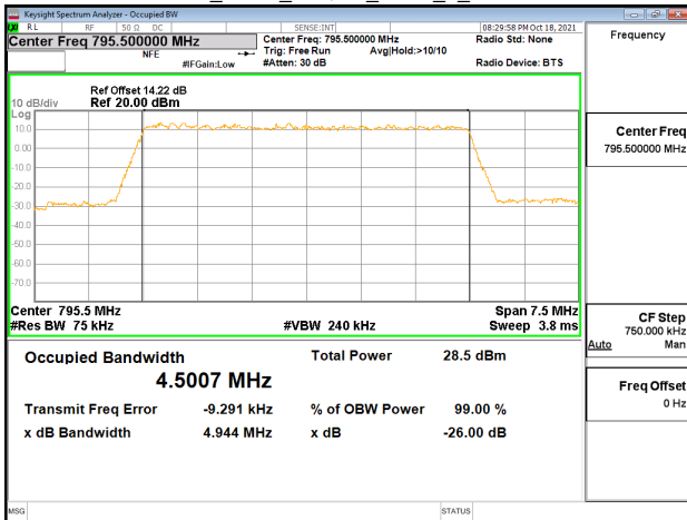
Band14_5MHz_64QAM_RB25_0_CH23355
