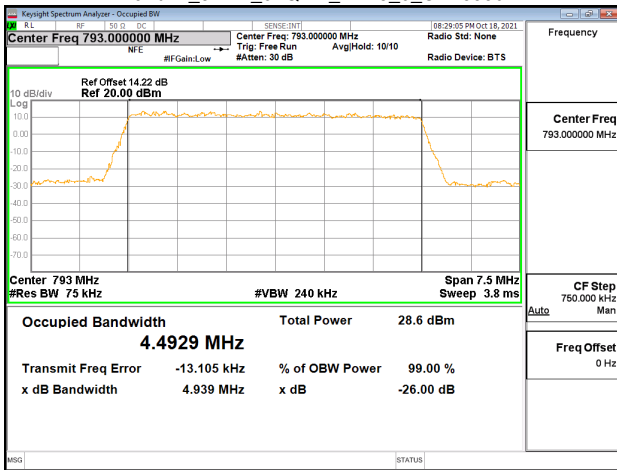
Band14_5MHz_64QAM_RB25_0_CH23355
