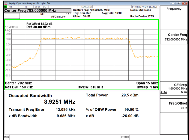
Band13_10MHz_64QAM_RB50_0_CH23230
