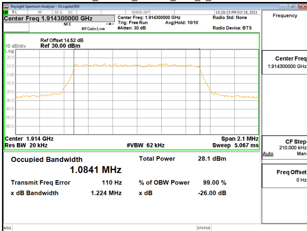
Band25_1.4MHz_64QAM_RB6_0_CH26683
