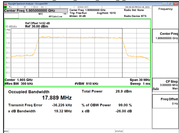
Band25_20MHz_64QAM_RB100_0_CH26590
