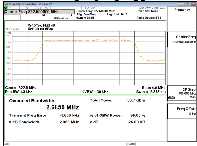
Band26-Part90s 3MHz QPSK_RB15_0_CH26775
