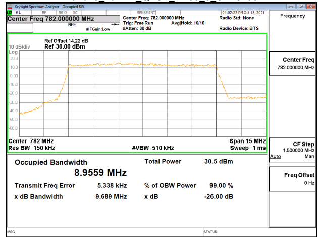
Band13_10MHz_16QAM_RB50_0_CH23230
