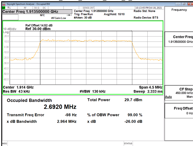
Band25_3MHz_16QAM_RB15_0_CH26675
