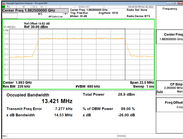
Band25_15MHz_64QAM_RB75_0_CH26615
