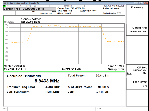
Band14_10MHz_16QAM_RB50_0_CH23330
