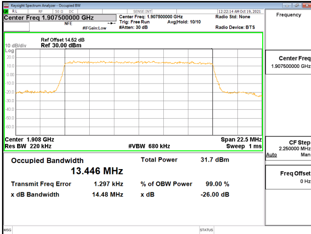
Band25_15MHz_QPSK_RB75_0_CH26615
