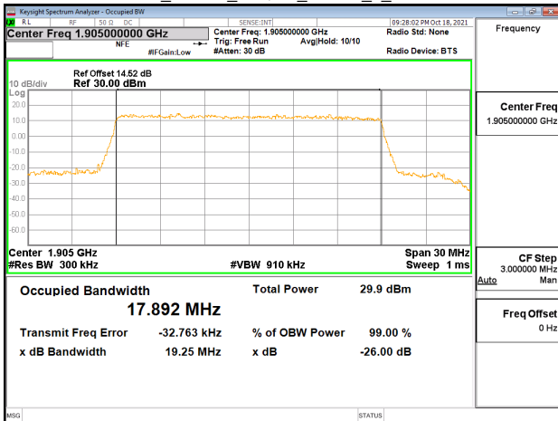
Band25_20MHz_16QAM_RB100_0_CH26590
