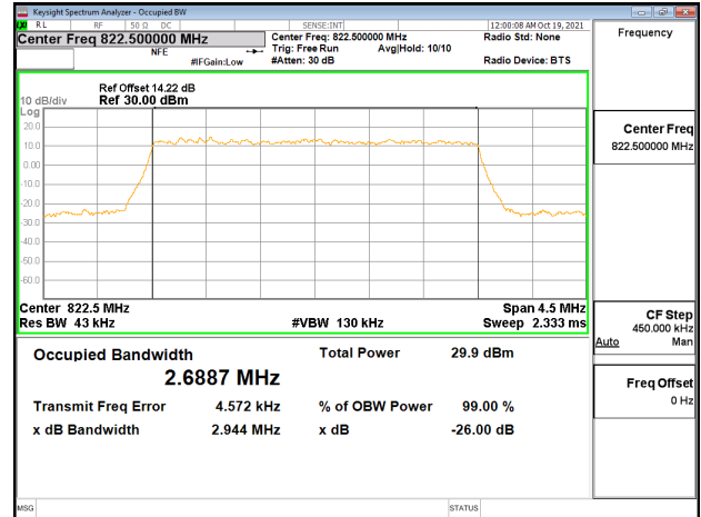
Band26-Part90s_3MHz_64QAM_RB15_0_CH26775
