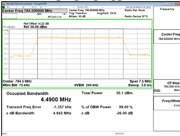
Band13_5MHz_QPSK_RB25_0_CH23255
