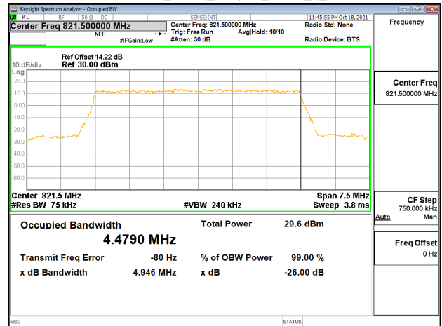
Band26-Part90s_5MHz_16QAM_RB25_0_CH26765
