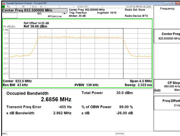
Band26-Part90s_3MHz_16QAM_RB15_0_CH26775
