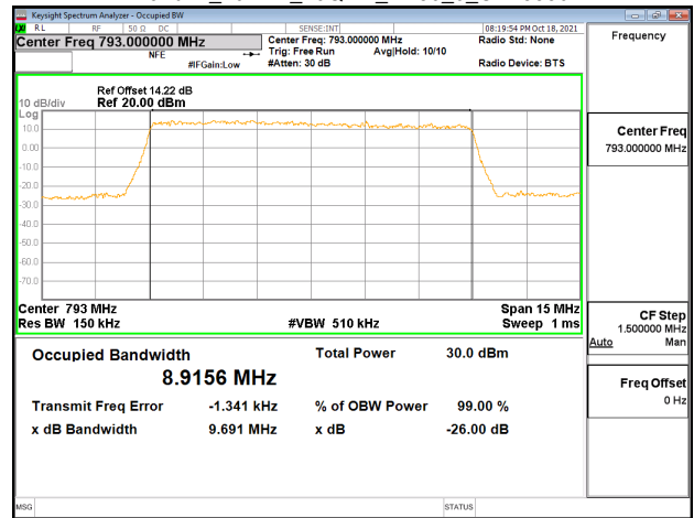
Band14_10MHz_64QAM_RB50_0_CH23330
