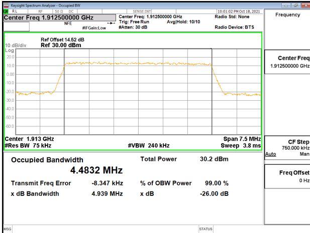
Band25_5MHz_QPSK_RB25_0_CH26665
