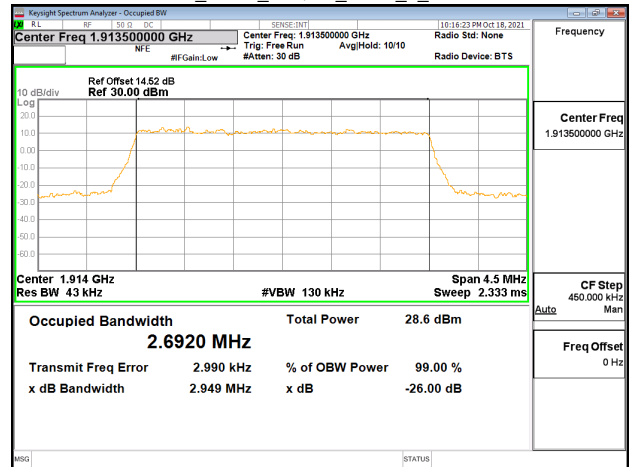
Band25_3MHz_64QAM_RB15_0_CH26675
