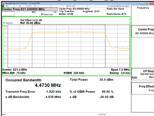
Band26-Part90s_5MHz_QPSK_RB25_0_CH26765
