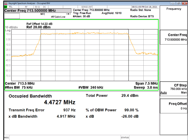
Band17_5MHz_16QAM_RB25_0_CH23825
