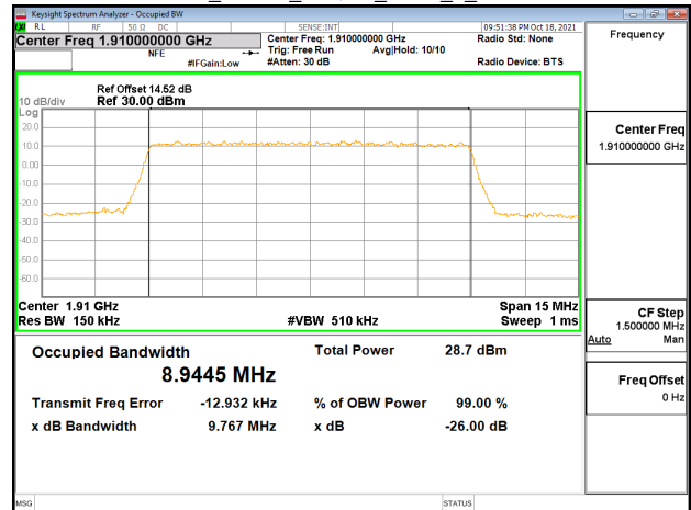
Band25_10MHz_64QAM_RB50_0_CH26640
