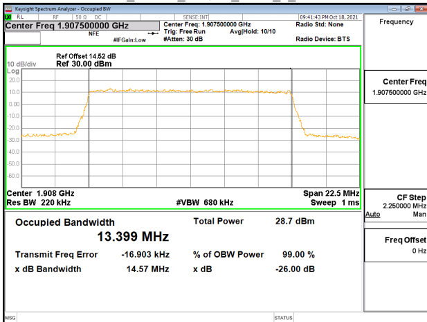
Band25_15MHz_64QAM_RB75_0_CH26615
