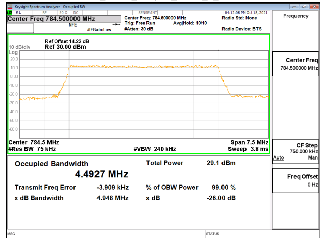
Band13_5MHz_16QAM_RB25_0_CH23255
