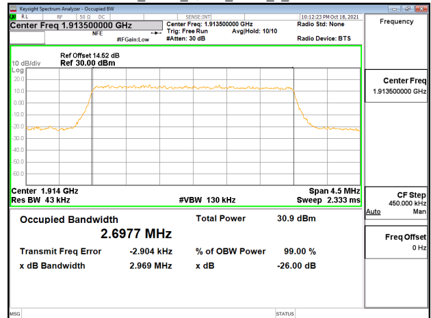
Band25_3MHz_QPSK_RB15_0_CH26675
