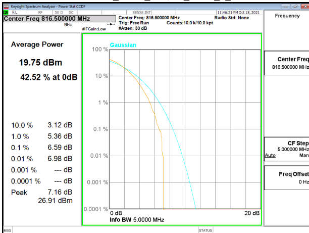
Band26-Part90s_5MHz_64QAM_RB25_0_CH26715
