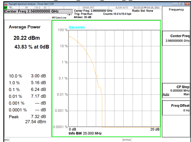
Band7_20MHz_64QAM_RB100_0_CH21350
