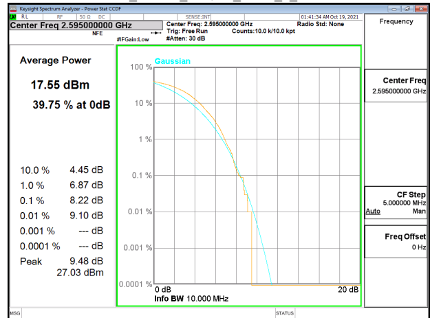
Band38_10MHz_64QAM_RB50_0_CH38000
