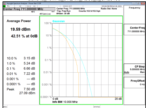
Band12_10MHz_64QAM_RB50_0_CH23130
