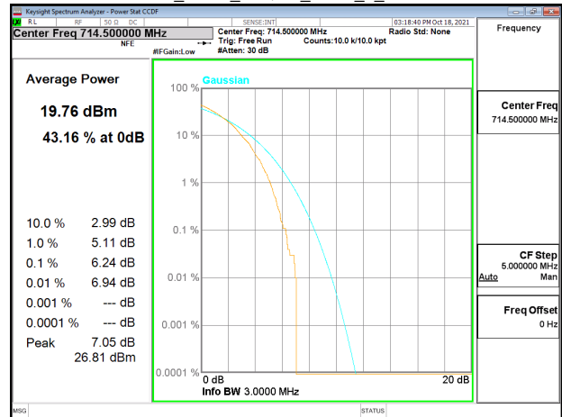
Band12_3MHz_64QAM_RB15_0_CH23165
