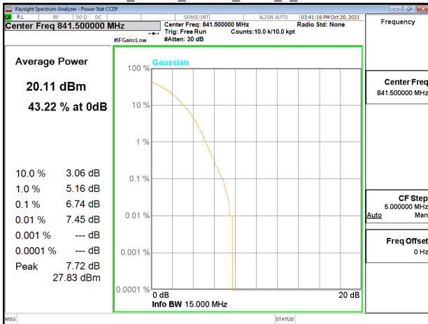
Band26_15MHz_64QAM_RB75_0_CH26965
