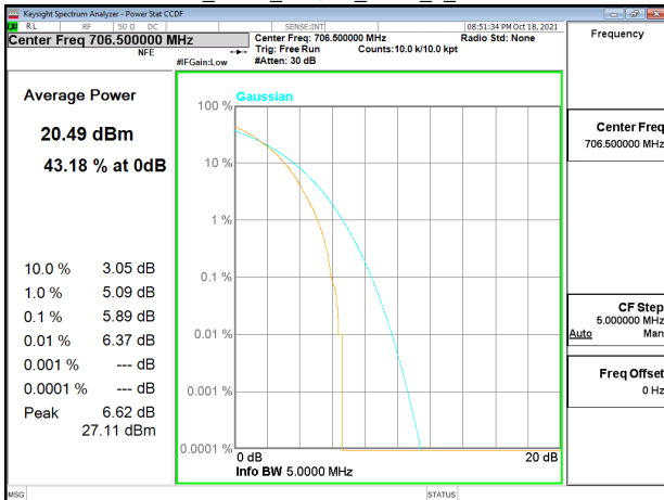
Band17_5MHz_64QAM_RB25_0_CH23755
