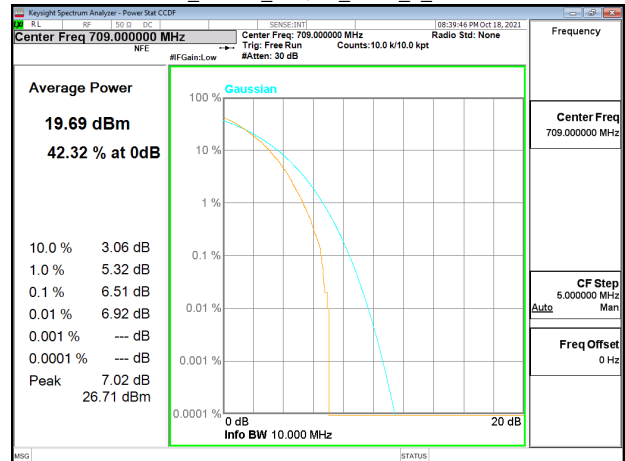
Band17_10MHz_64QAM_RB50_0_CH23780
