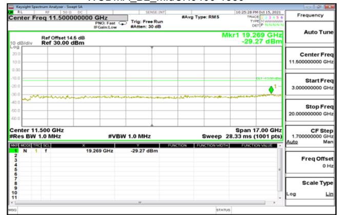
WCDMA_B2_HighCH9538-1907.6
