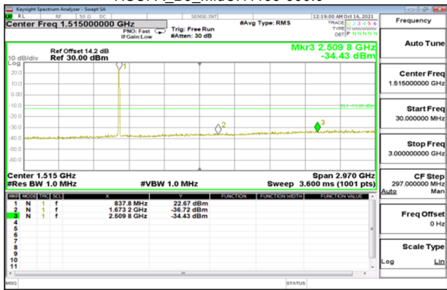
HSUPA_B5_HighCH4233-846.6
