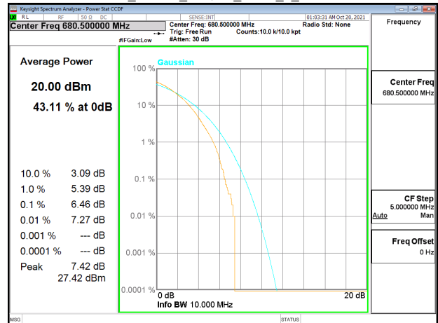
Band71_10MHz_64QAM_RB50_0_CH133297
