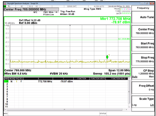
Band13_5MHz_QPSK_RB1_24_CH23255
