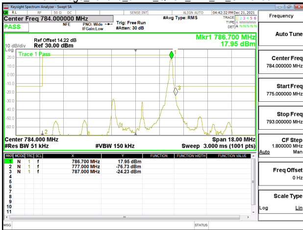
Band Edge_Band13_5MHz_QPSK_RB25_0_CH23205
