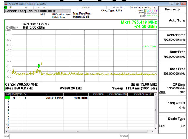
Band13_5MHz_QPSK_RB25_0_CH23205
