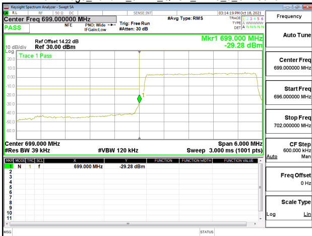
Band Edge_Band12_3MHz_QPSK_RB15_0_CH23025
