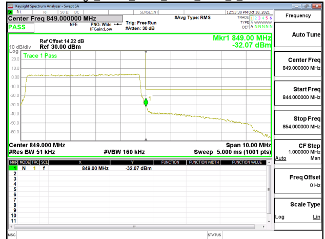
Band Edge_Band5_5MHz_QPSK_RB25_0_CH20625
