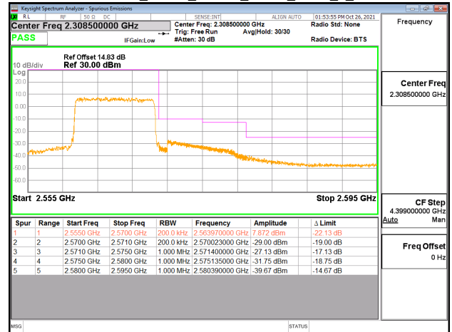
Emission Mask_Band7_10MHz_QPSK_RB50_0_CH21400
