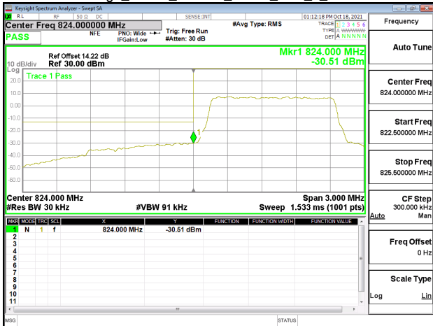
Band Edge_Band5_1.4MHz_QPSK_RB6_0_CH20407
