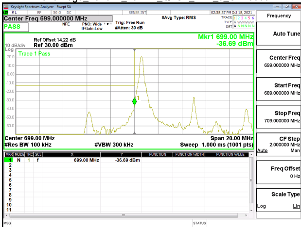
Band Edge_Band12_10MHz_QPSK_RB1_0_CH23060
