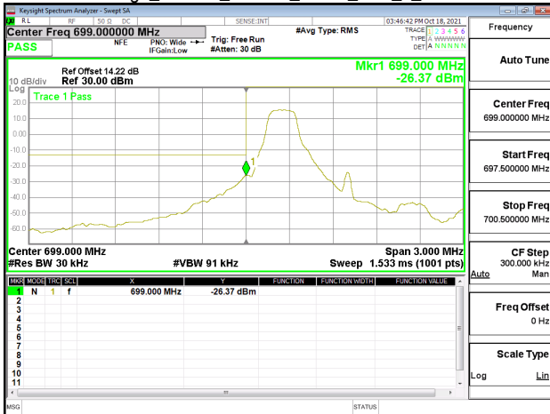
Band Edge_Band12_1.4MHz_QPSK_RB1_0_CH23017
