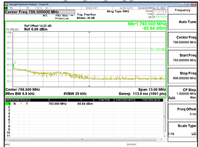
Band13_5MHz_QPSK_RB25_0_CH23255
