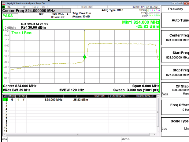
Band Edge_Band5_3MHz_QPSK_RB15_0_CH20635
