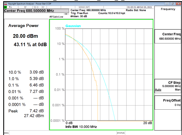
Band71_10MHz_64QAM_RB50_0_CH133297
