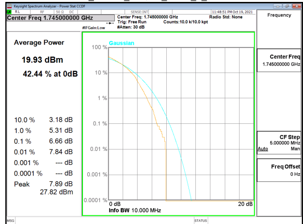
Band66_10MHz_64QAM_RB50_0_CH132322
