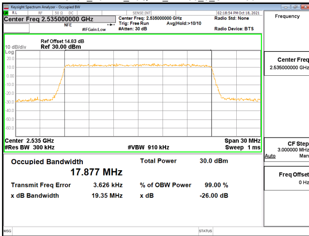
Band7_20MHz_16QAM_RB100_0_CH21350
