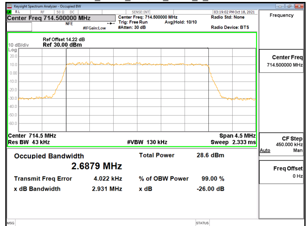
Band12_3MHz_64QAM_RB15_0_CH23165
