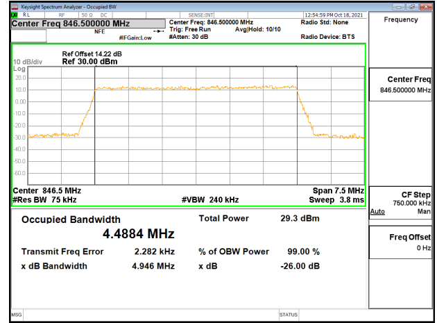
Band5_5MHz_16QAM_RB25_0_CH20625
