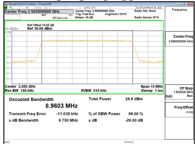
Band7_10MHz_64QAM_RB50_0_CH21400
