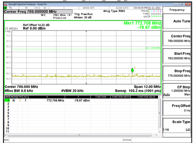
Band13_5MHz_QPSK_RB1_24_CH23255
