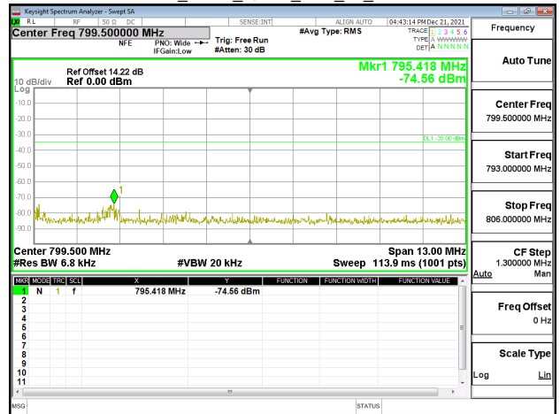
Band13_5MHz_QPSK_RB25_0_CH23205
