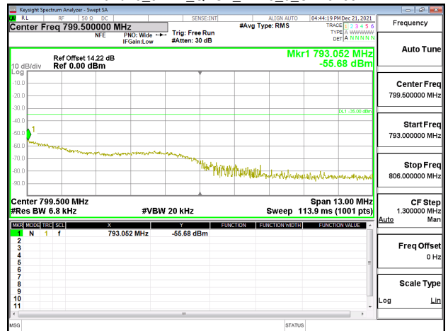
Band13_5MHz_QPSK_RB25_0_CH23255
