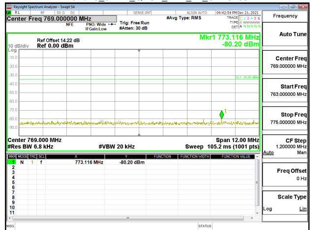
Band13_5MHz_QPSK_RB1_24_CH23255
