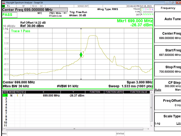
Band Edge_Band12_1.4MHz_QPSK_RB1_0_CH23017
