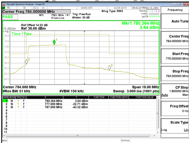
Band Edge_Band13_5MHz_QPSK_RB25_0_CH23205
