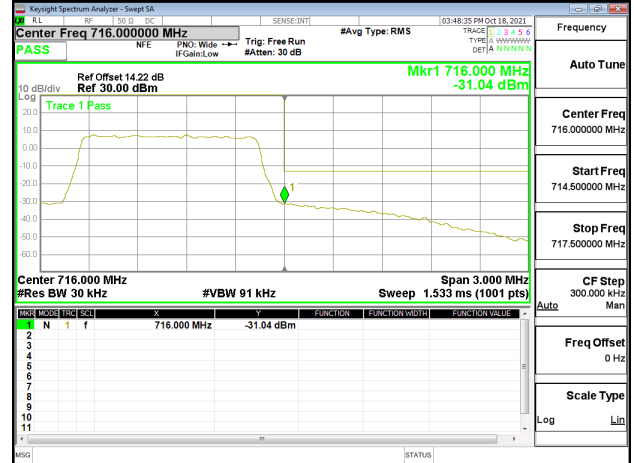
Band Edge_Band12_1.4MHz_QPSK_RB6_0_CH23173
