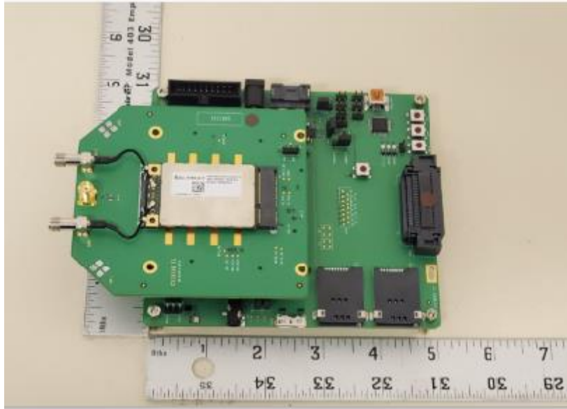
Figure B1. DUT Top View
