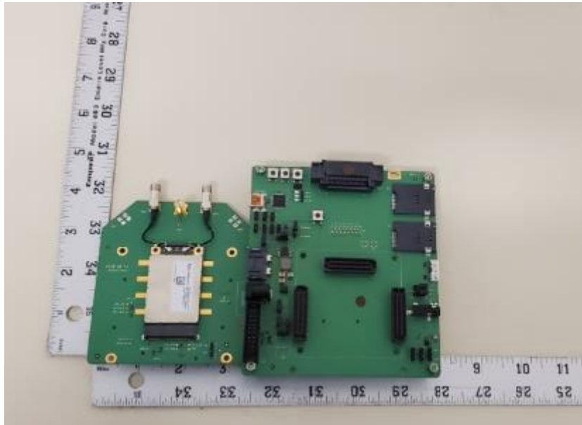
Figure B3. DUT Circuit board and module
