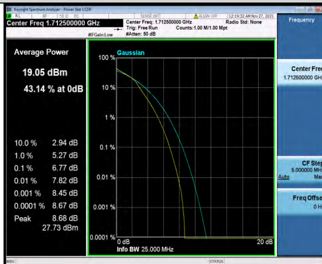
Band4-5MHz-16QAM-20175-1RB#0
