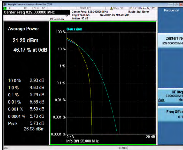
Band5-10MHz-16QAM-20450-27RB#0
