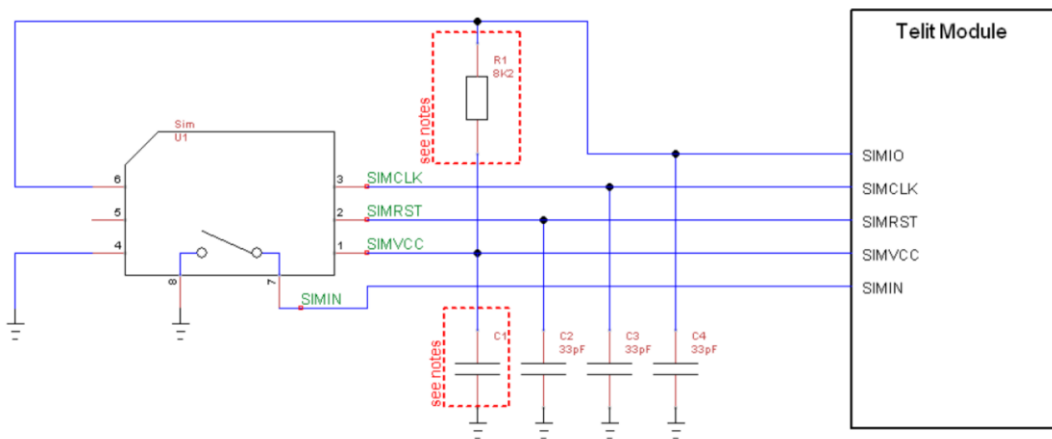
Figure 30: SIM Schematics
