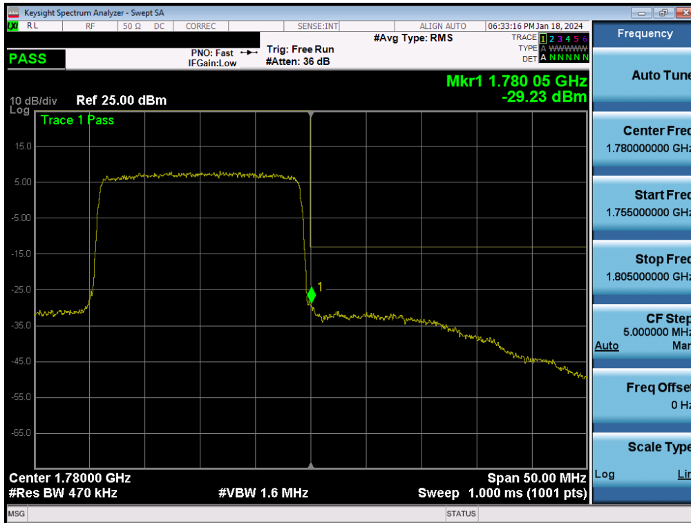
Plot 7-66. Upper Band Edge Plot (LTE Band 66 - 20MHz QPSK – Full RB)
