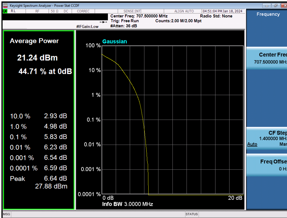
Plot 7-103. PAR Plot (LTE Band 12 - 3MHz 16-QAM - Full RB)
