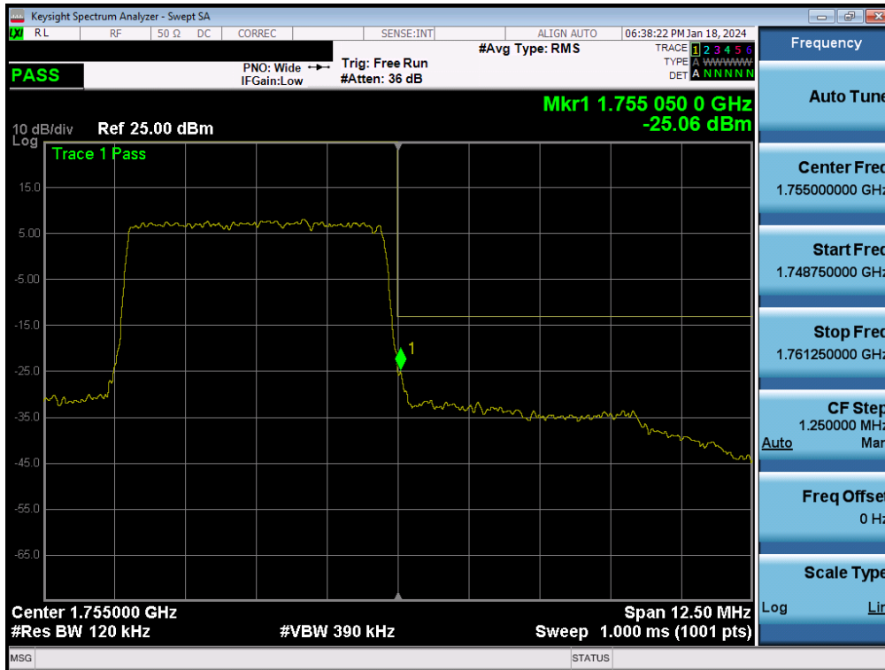
Plot 7-82. Upper Band Edge Plot (LTE Band 4 - 5MHz QPSK – Full RB)
