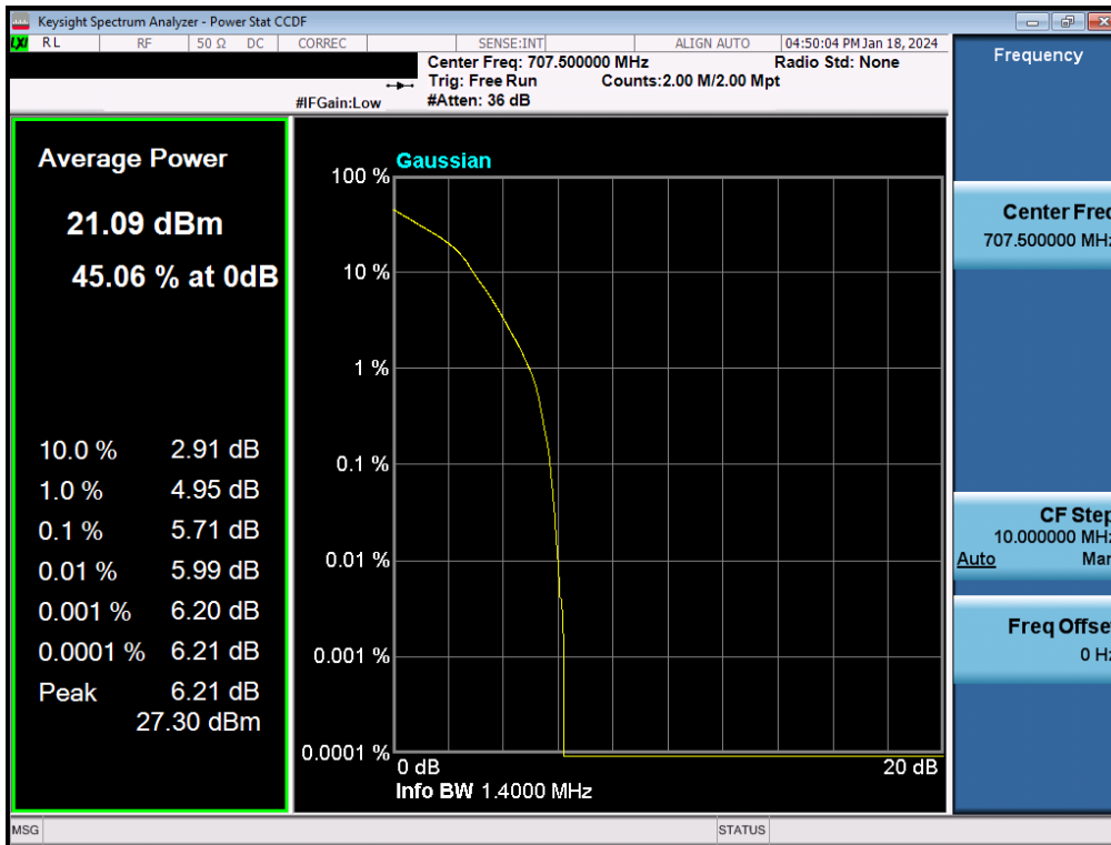
Plot 7-105. PAR Plot (LTE Band 12 - 1.4MHz 16-QAM - Full RB)
