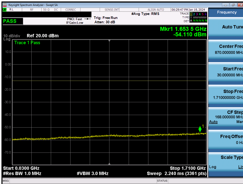
Plot 7-40. Conducted Spurious Plot (LTE Band 66/4 - 20MHz QPSK - 1 RB - Mid Channel)
