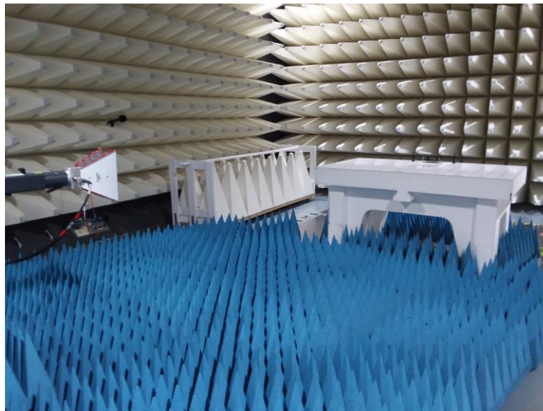
Figure B5. Radiated Setup HR
