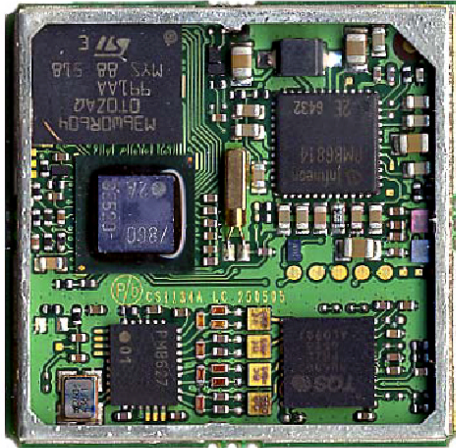
Photograph No.5 GE864-Quad module internal view
