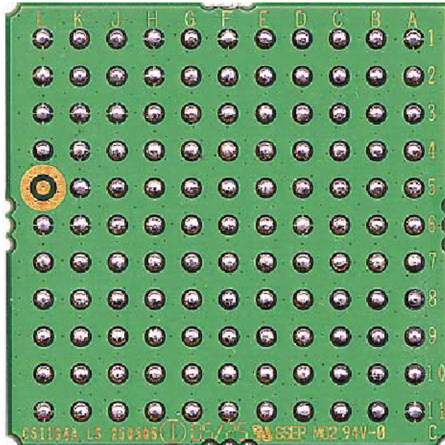
Photograph No.6 GE864-Quad module PCB second side view
