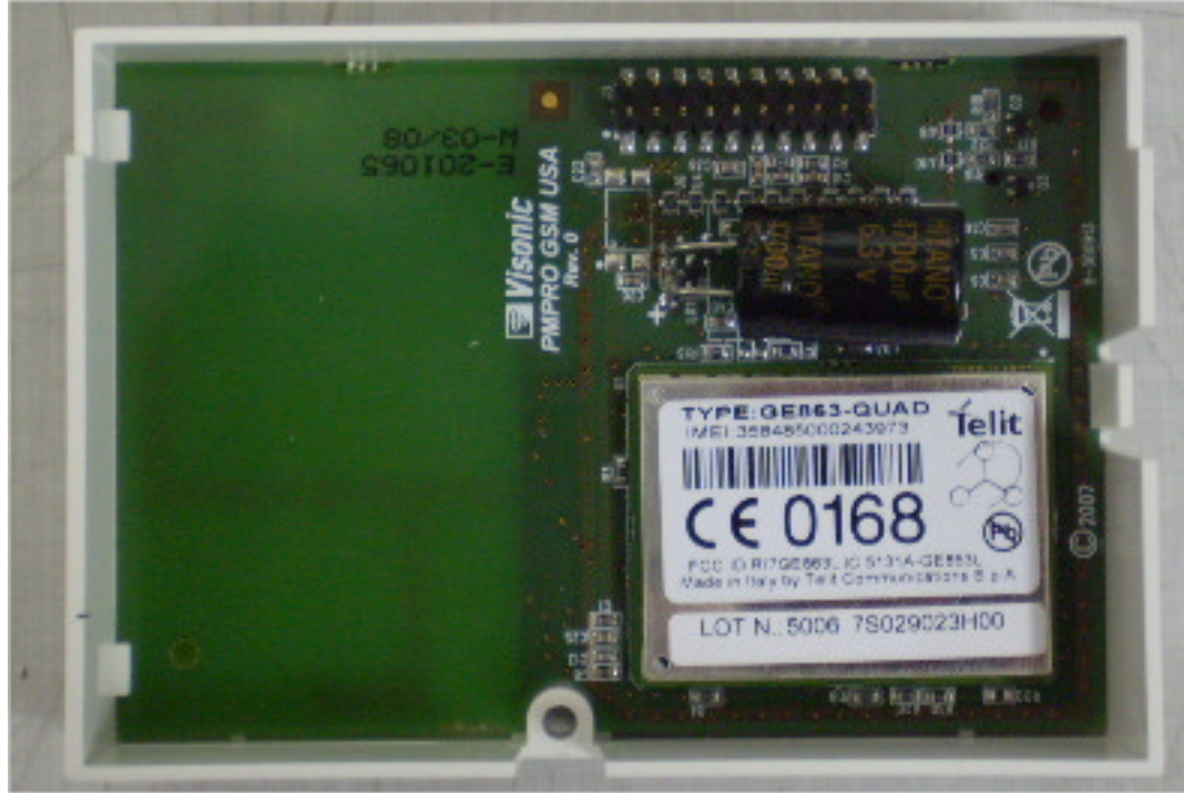
Photograph No.1 GSM module internal view
