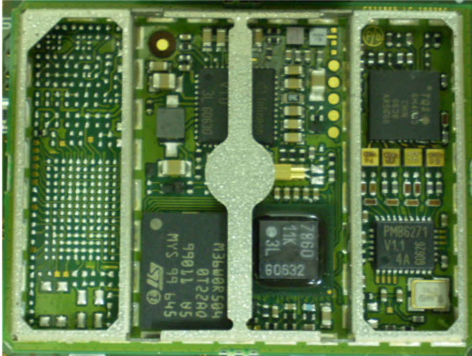
Photograph No.5 GE863-Quad module internal view
