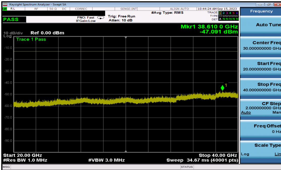
Plot 7-16. Conducted Spurious Plot (NR Band n78 - 10MHz QPSK - Mid Channel)
