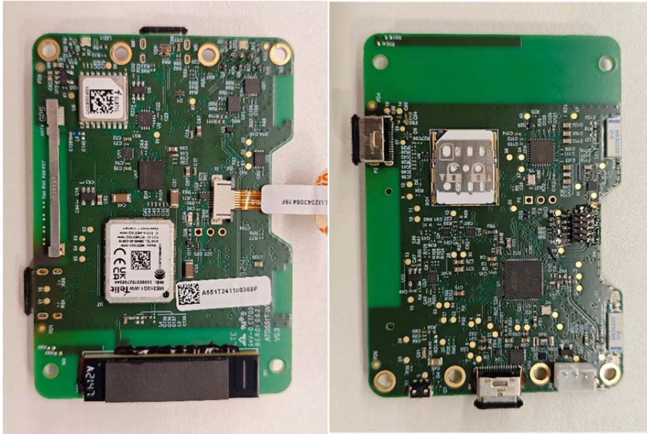
Figure 5: PCBA board
