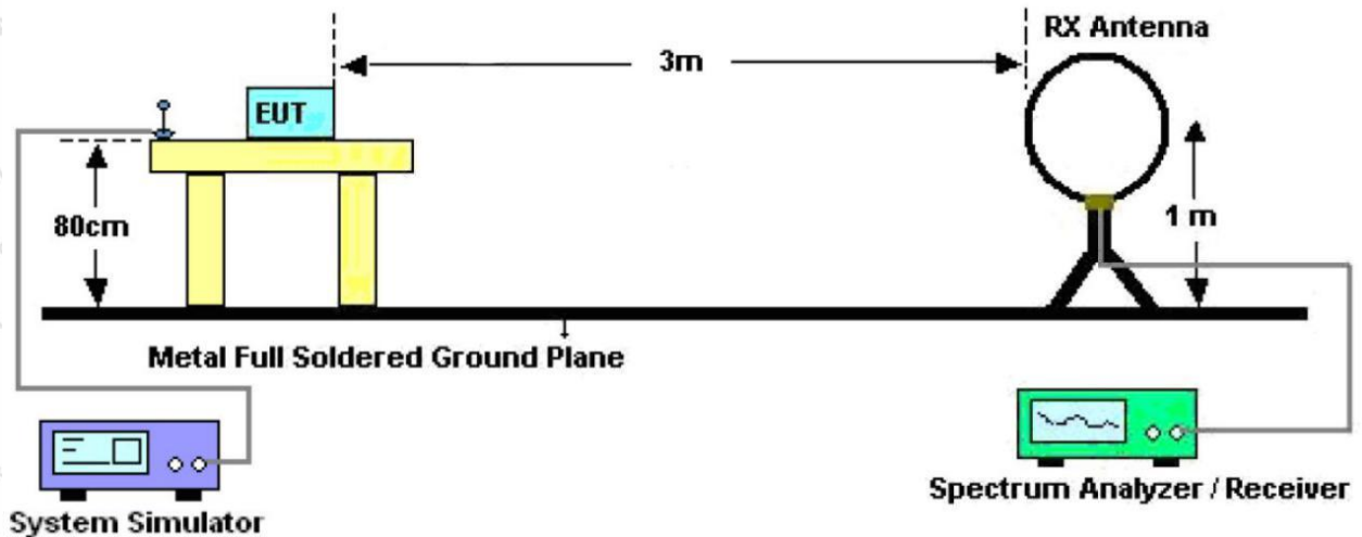
Figure 1. Below 30MHz
