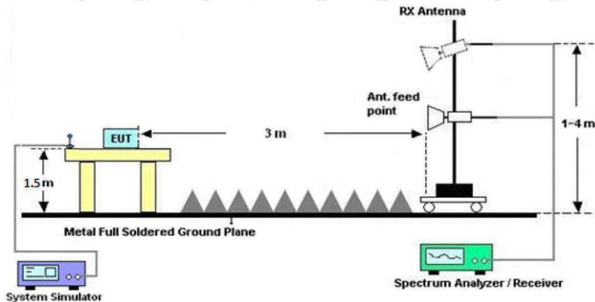
Figure 3. Above 1 GHz
