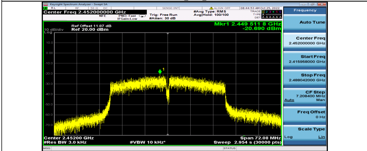
11N40SISO_Ant1_2452
