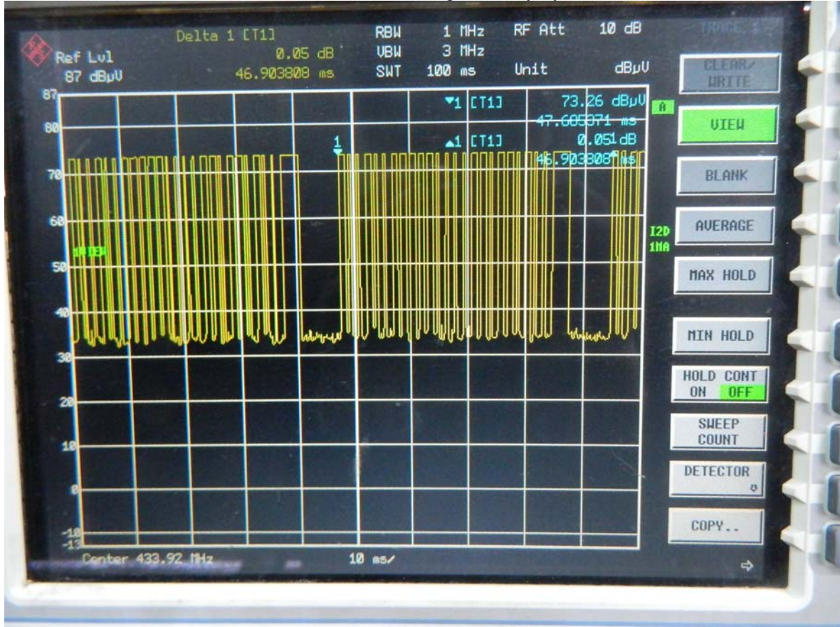
Pulse train with the highest duty cycle
