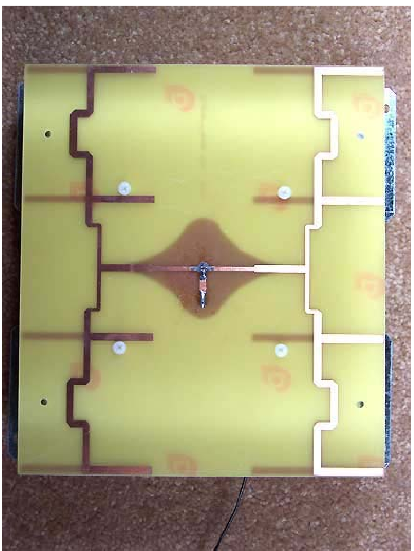
Antenna 2 Directional Front
