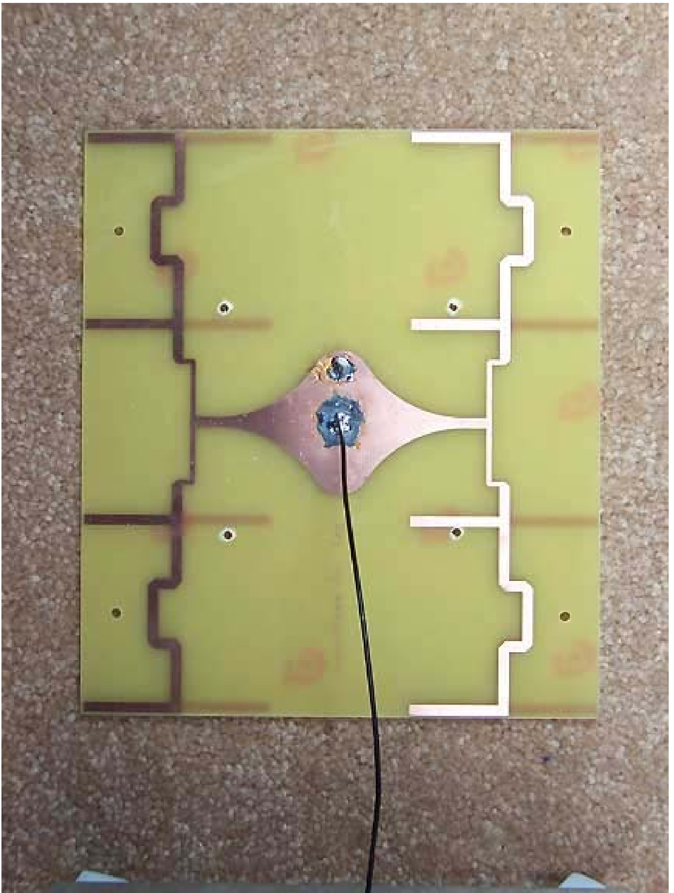
Antenna 2 directional back
