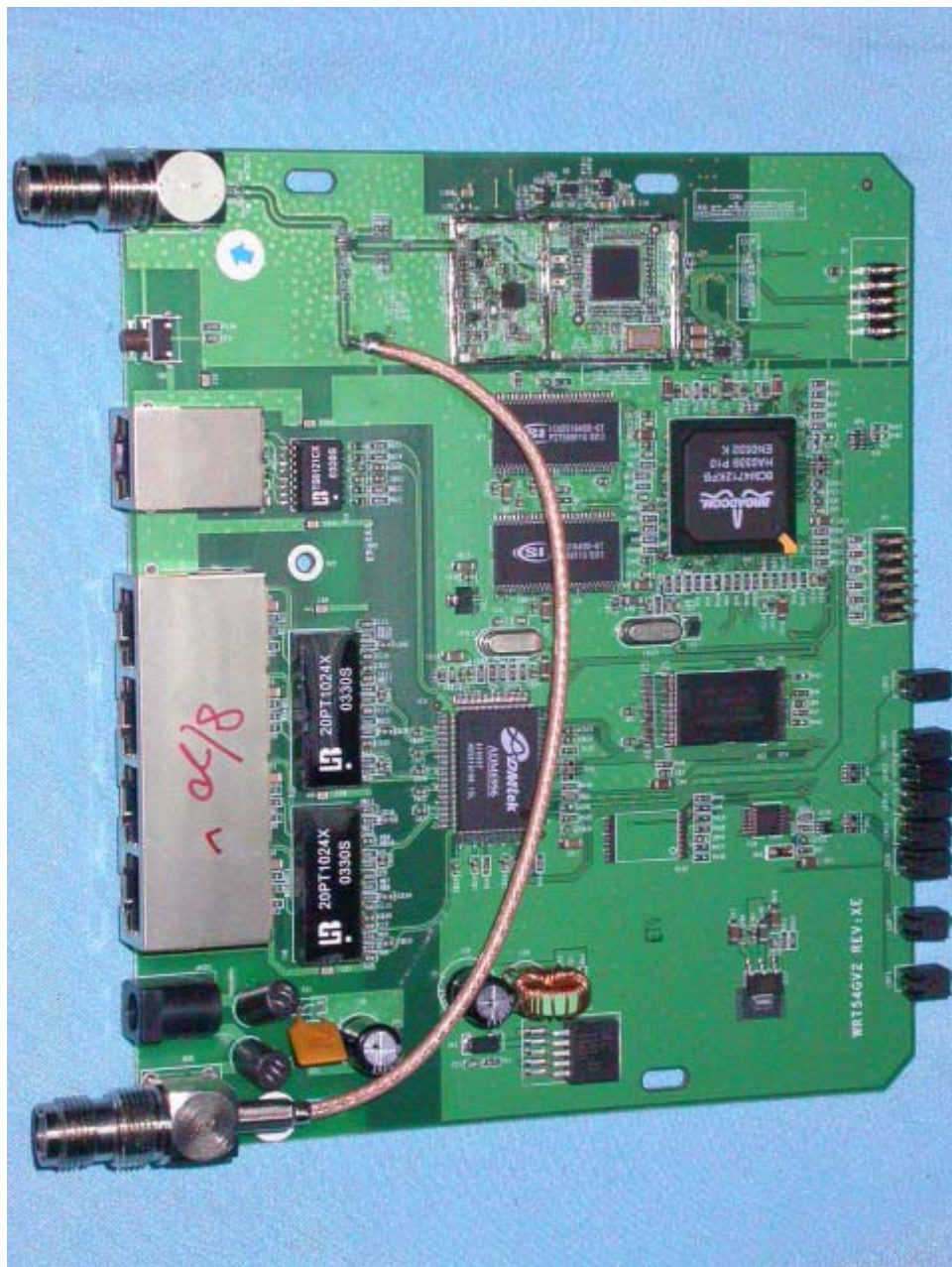
PCB Front Side Photo
