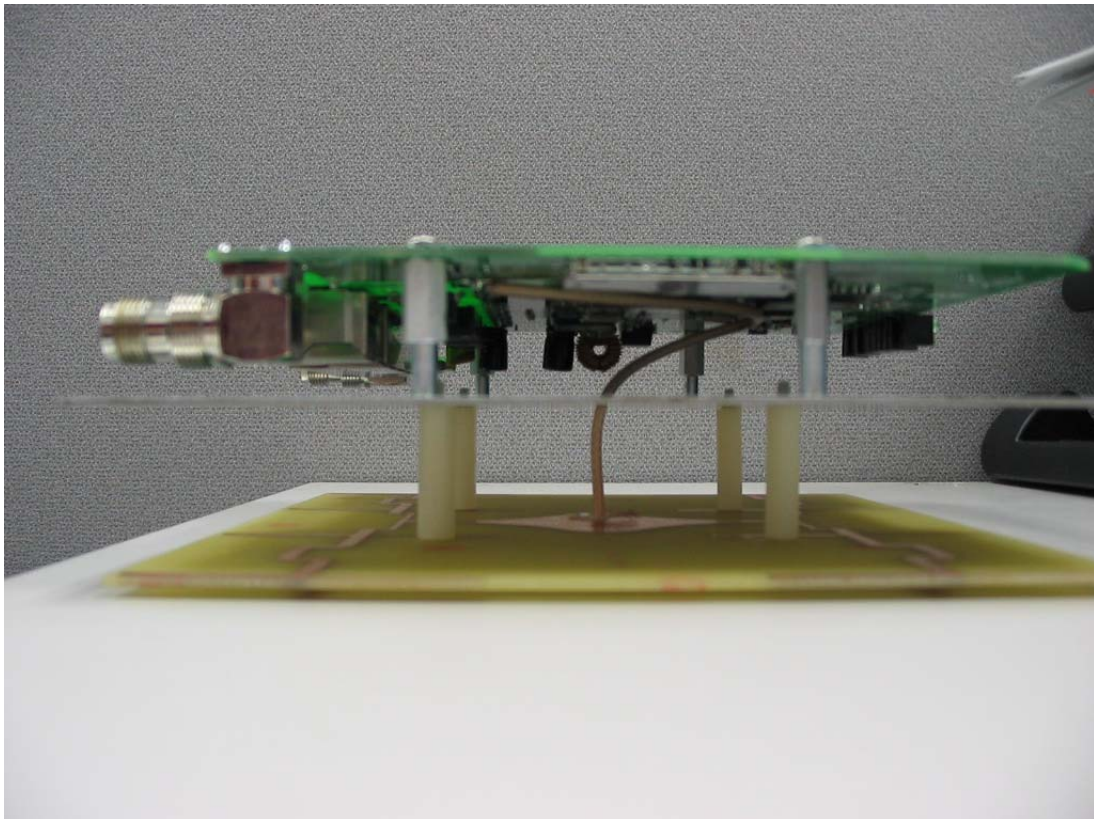
Assembled PCB w/ direct solder to Antenna Side view
