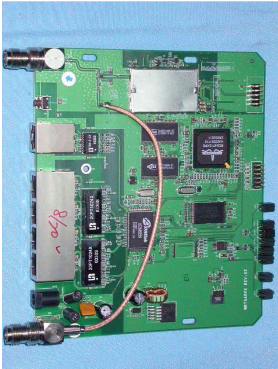
PCB Front
