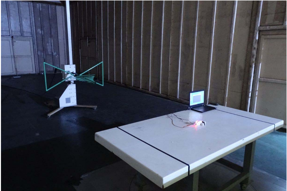
Back View of Radiated Test
