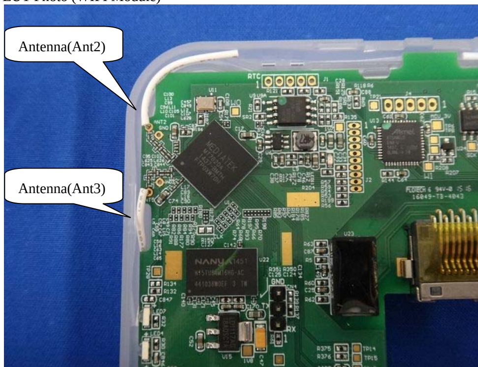
(14) EUT Photo (WIFI Module)
