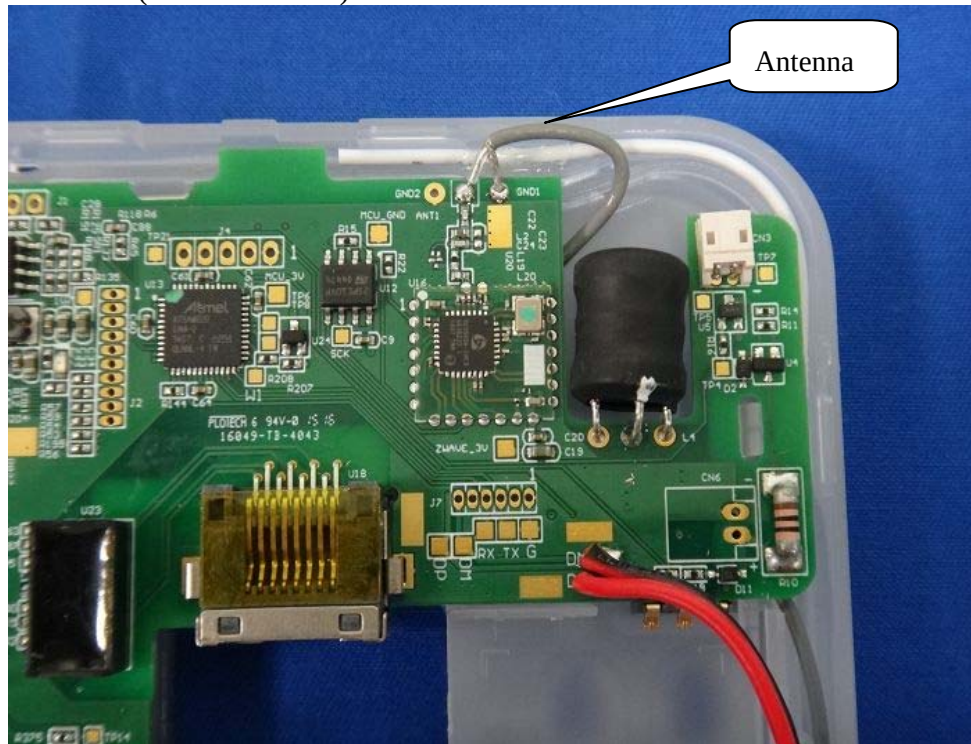
(13) EUT Photo(Z-Wave Module)
