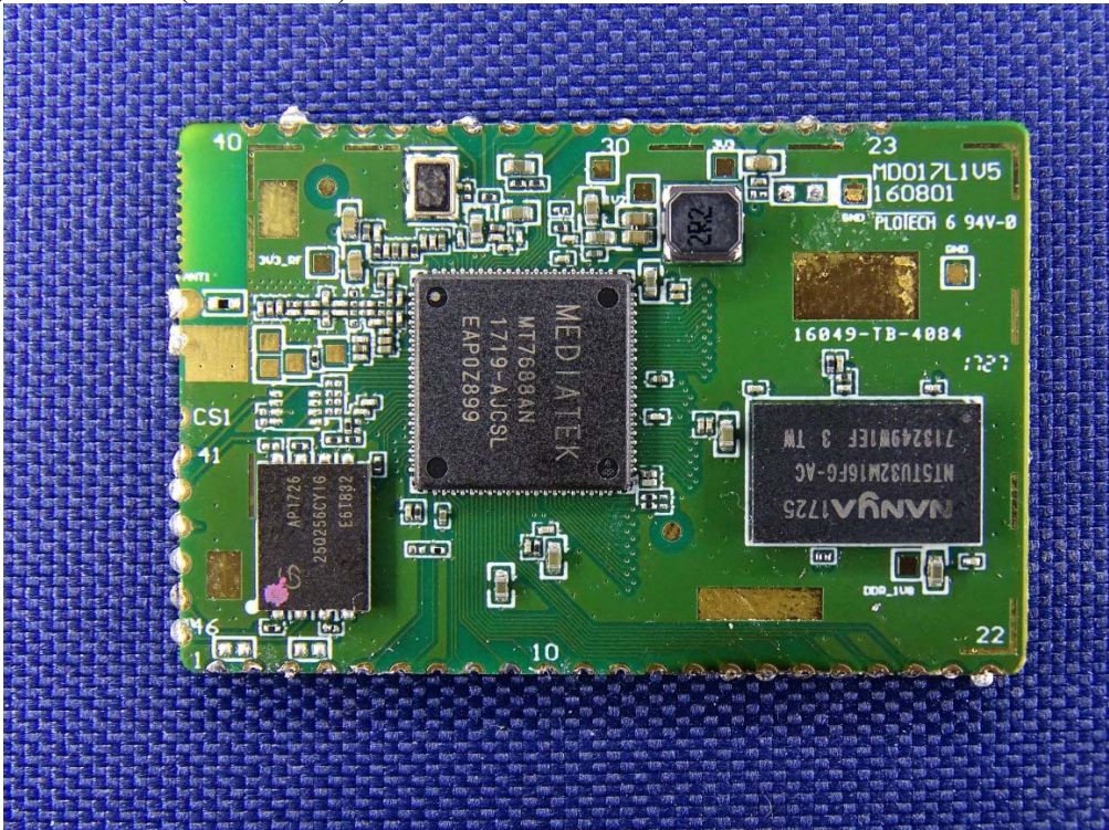
(25) EUT Photo (RF Module)
