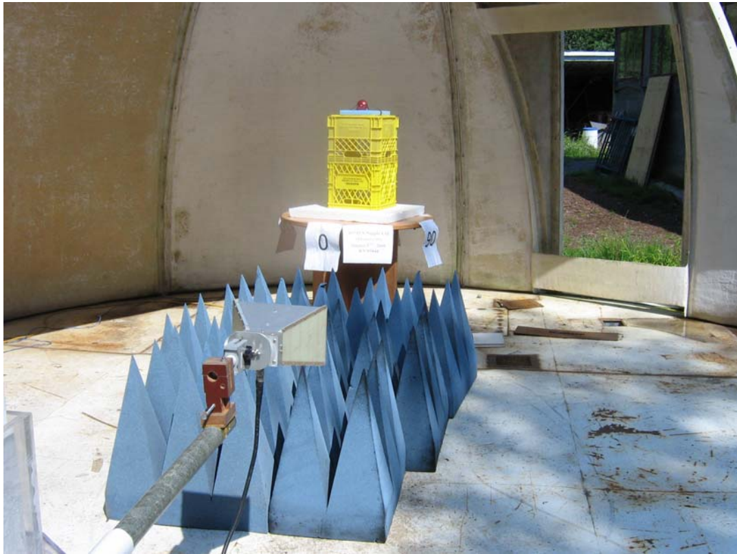
Pic 3: Emissions Test Setup of EUT during Radiated Emissions Testing
