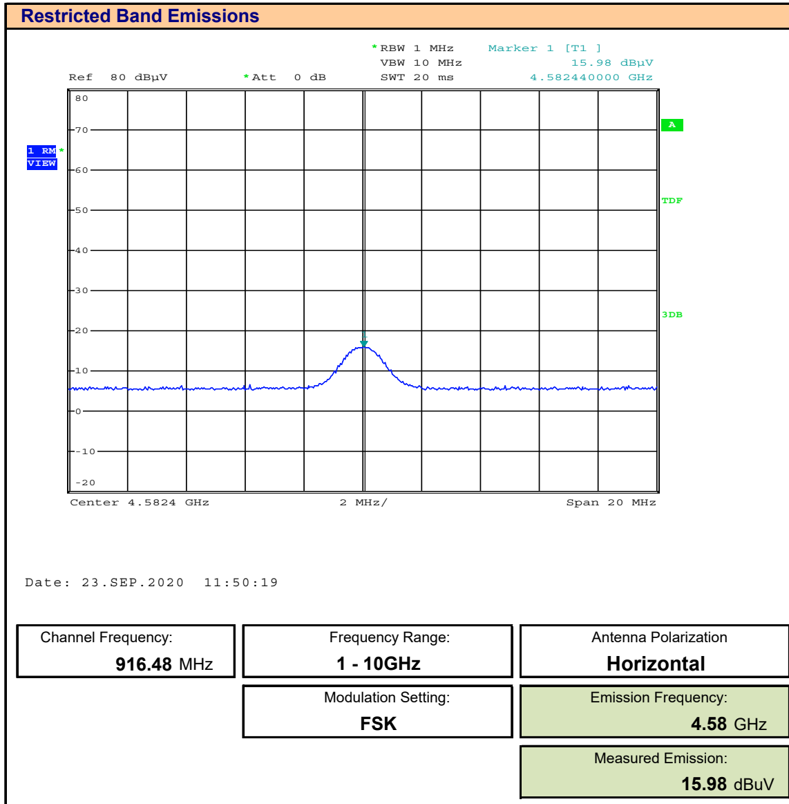
Plot 10.11 – Restricted Band, 5 th Harmonic, Horizontal
