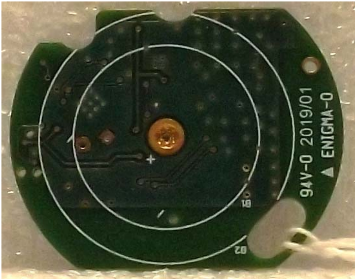
Figure E20.3 – Internal Photo – PCB Bottom, Battery Removed
