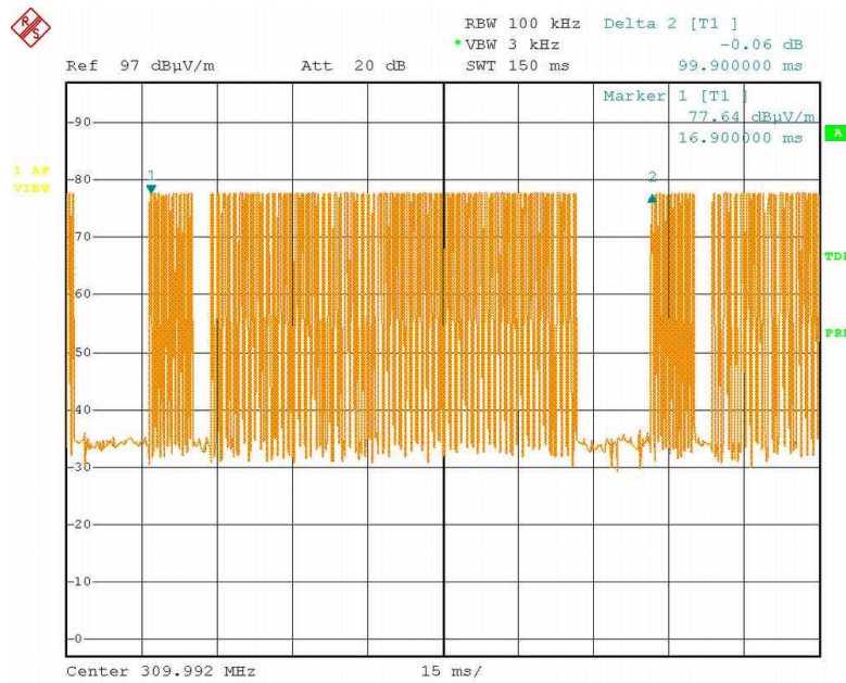
Duty Cycle Detail, Over a 100 ms Interval
