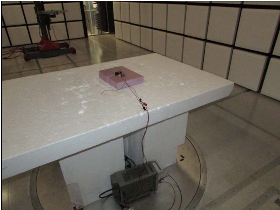
Figure 3: Radiated Emissions – Below 1GHz – Back
