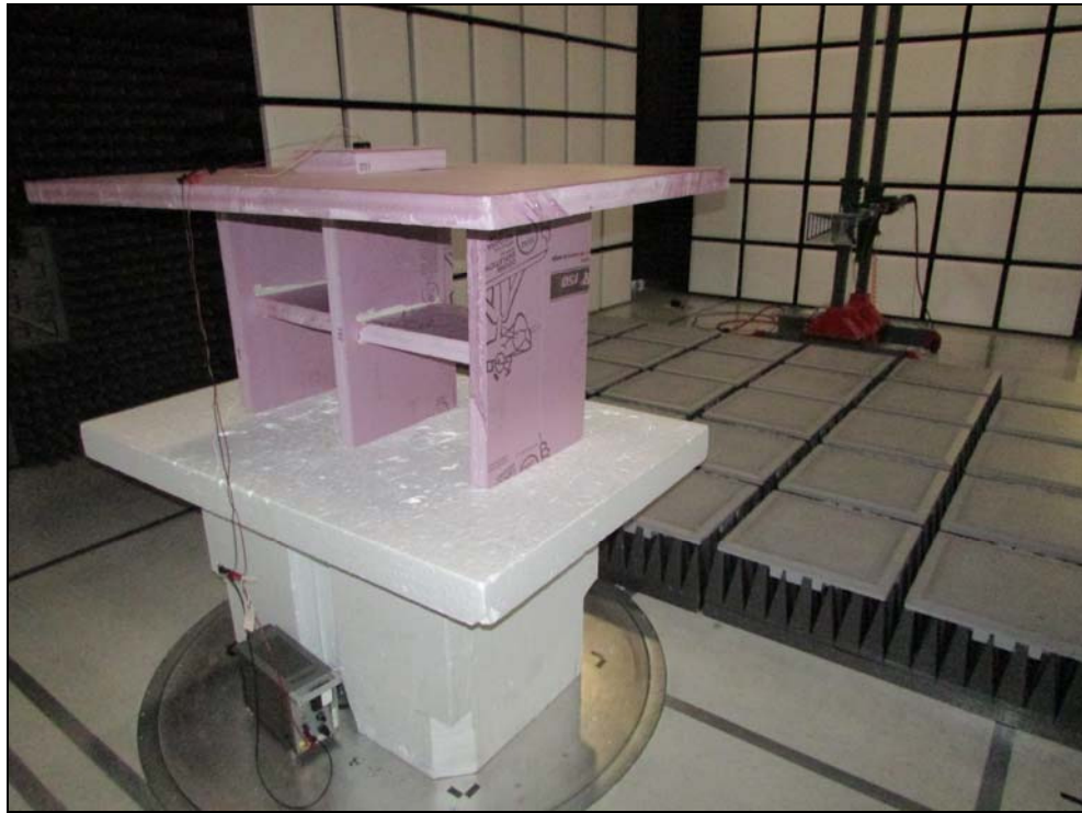
Figure 1: Radiated Emissions – Above 1GHz – Back
