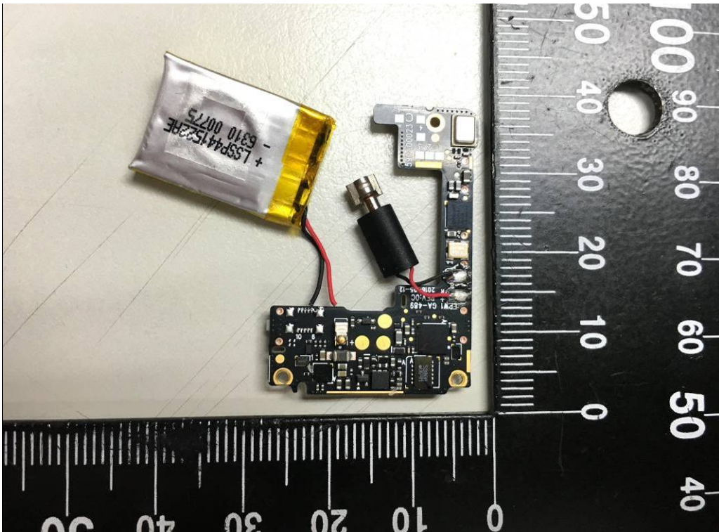
Battery
