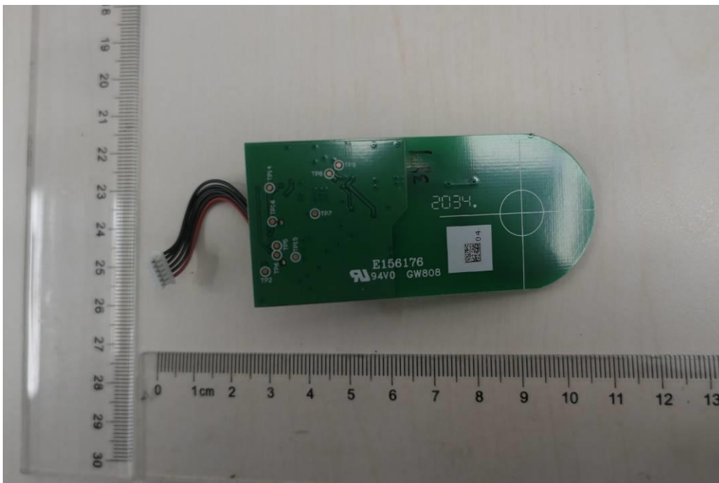
Fig 15: NFC PCB bottom view
