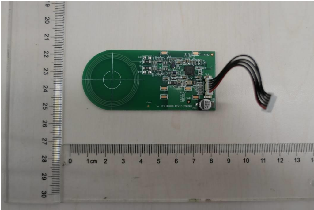
Fig 14: NFC PCB top view
