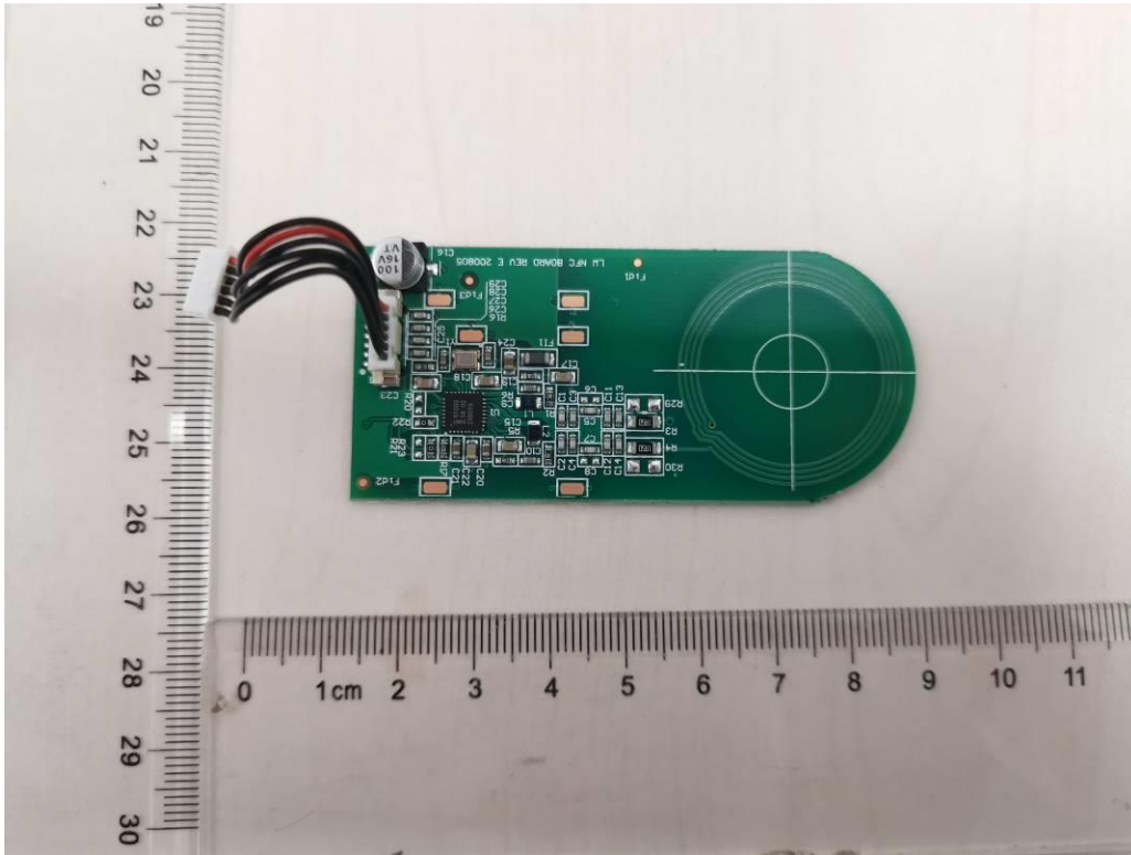
Fig 14: NFC PCB top view
