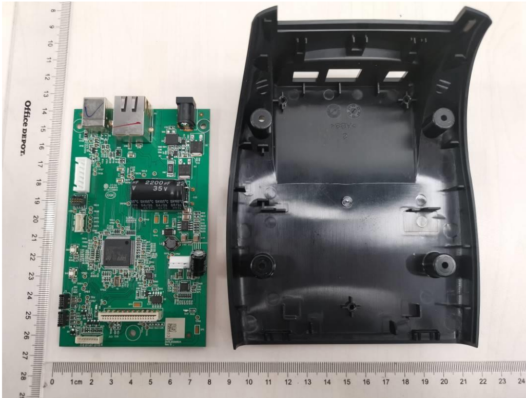
Fig 12: Main PCB top view
