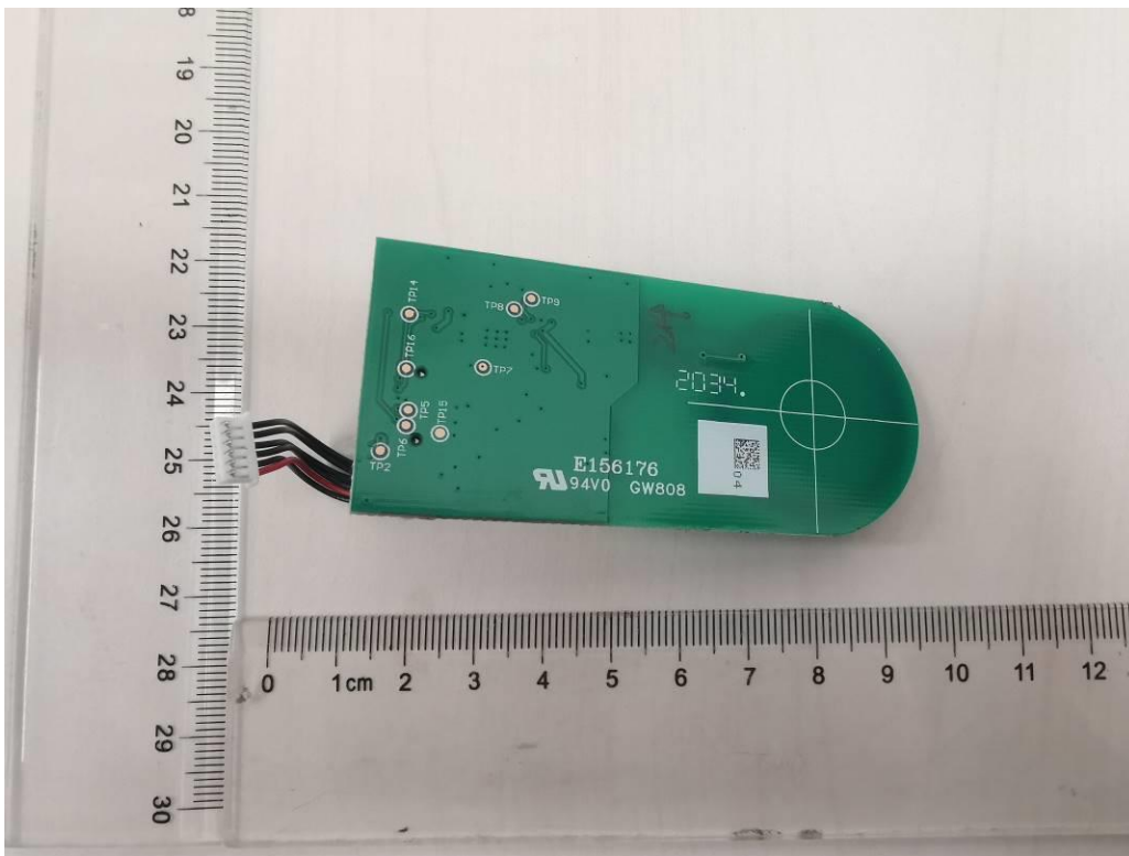
Fig 15: NFC PCB bottom view
