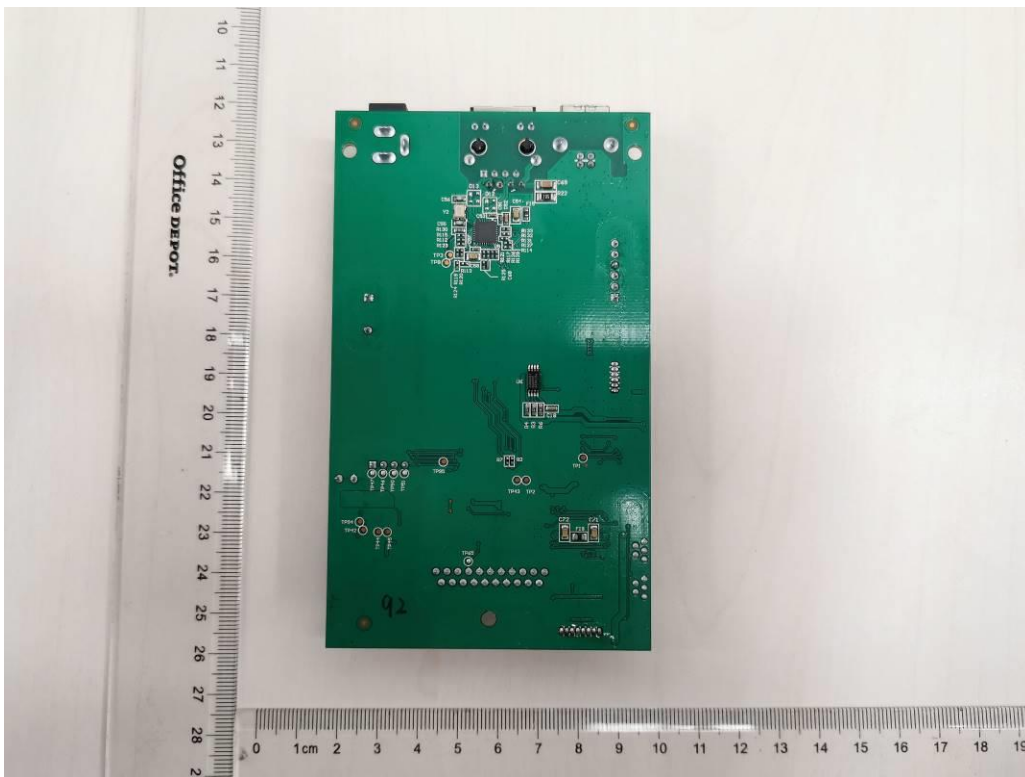
Fig 13: Main PCB bottom view
