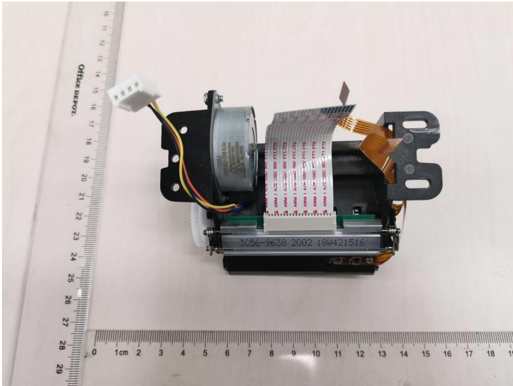
Fig 16: Print header top view
