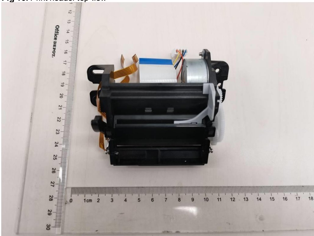
Fig 17: Print header bottom view
