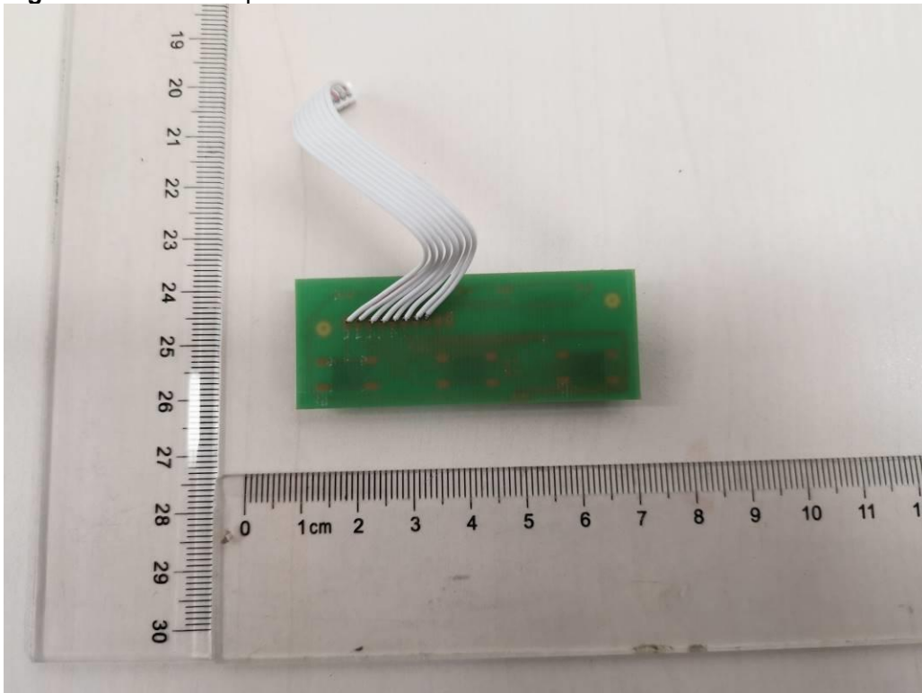
Fig 19: Button PCB bottom view
