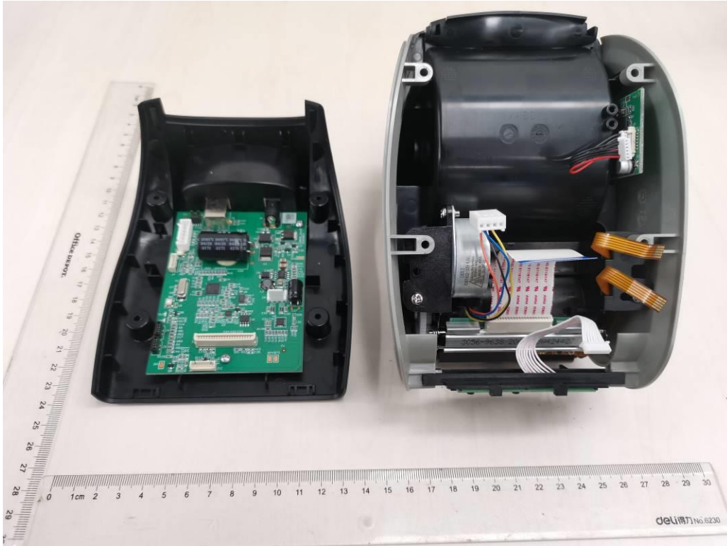
Fig 10: Internal view-3
