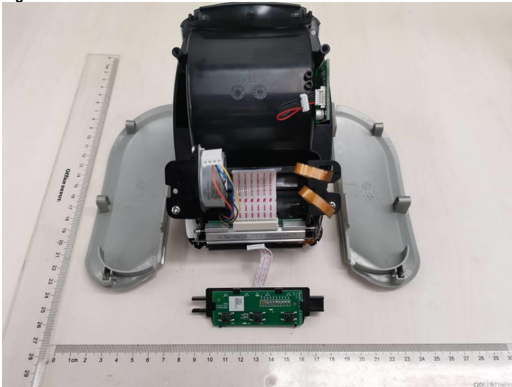
Fig 11: Internal view-4
