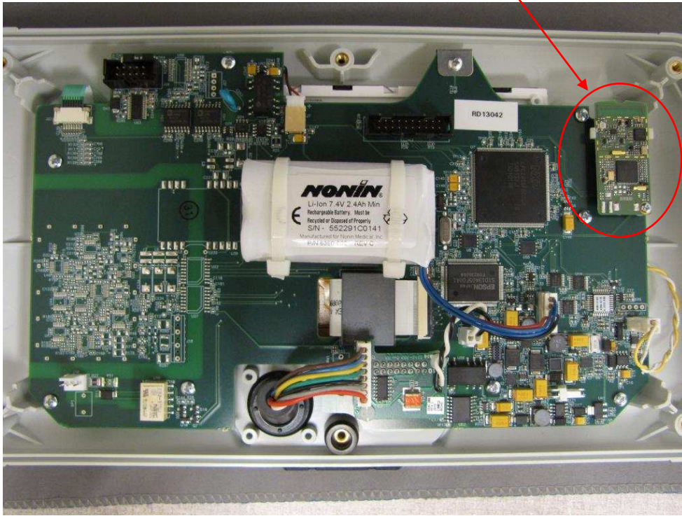
Figure 1 – Interior of Model 7600, showing main printed wire board assembly (PWBA) and Saber module
