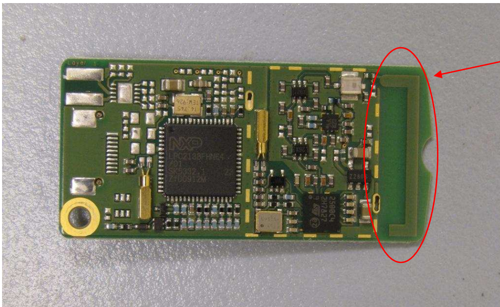
Figure 2 – Saber module PWBA (front) showing antenna
