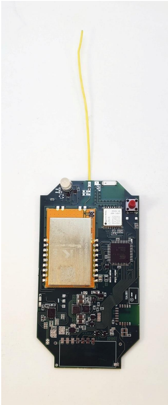
MMI-TRAKR1 – PCB, Front
