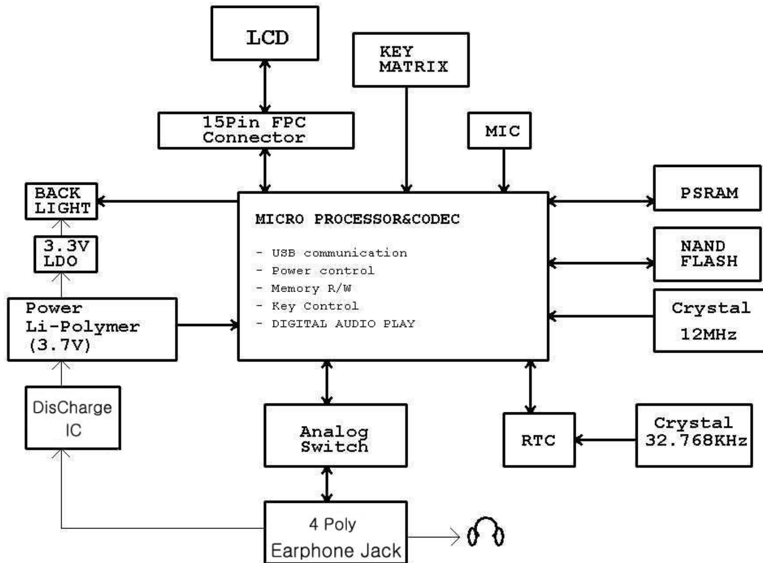
MPIO-PL300 Blockdiagram
