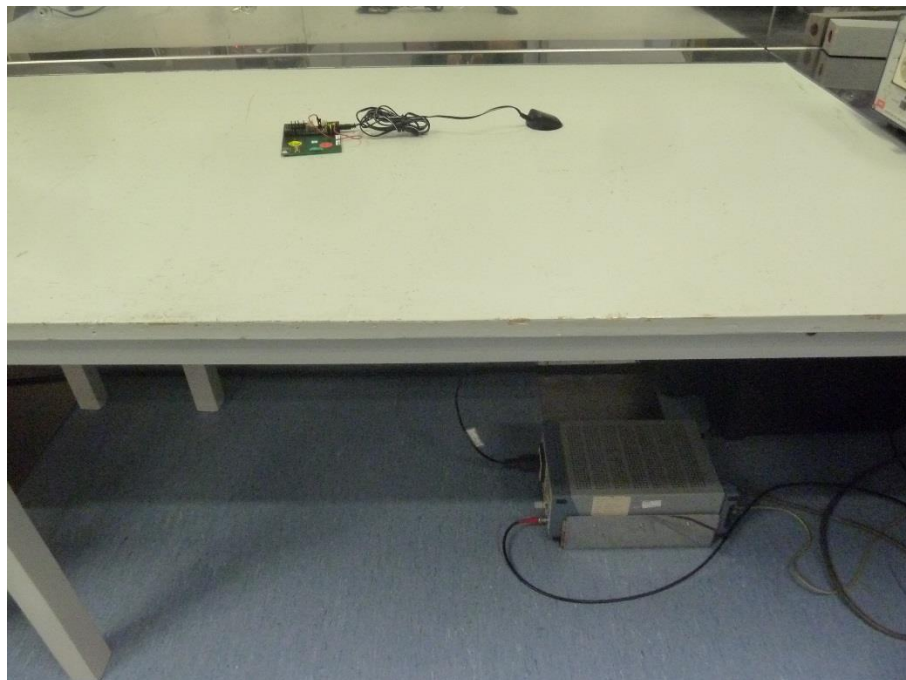
Photo 10: AC conducted
