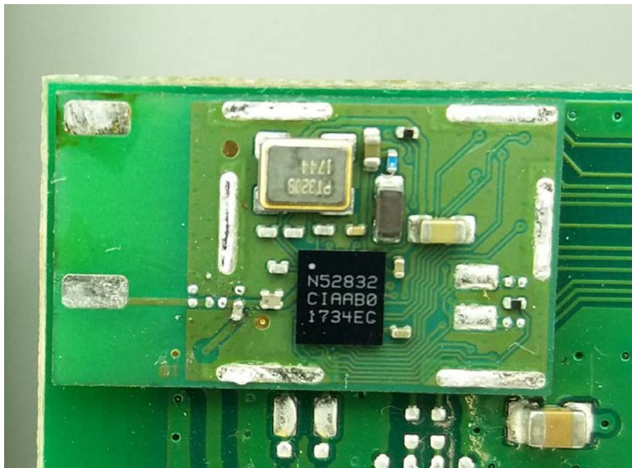
Photo 2: Module without shielding, PMN: BlueMod+S50/AP
