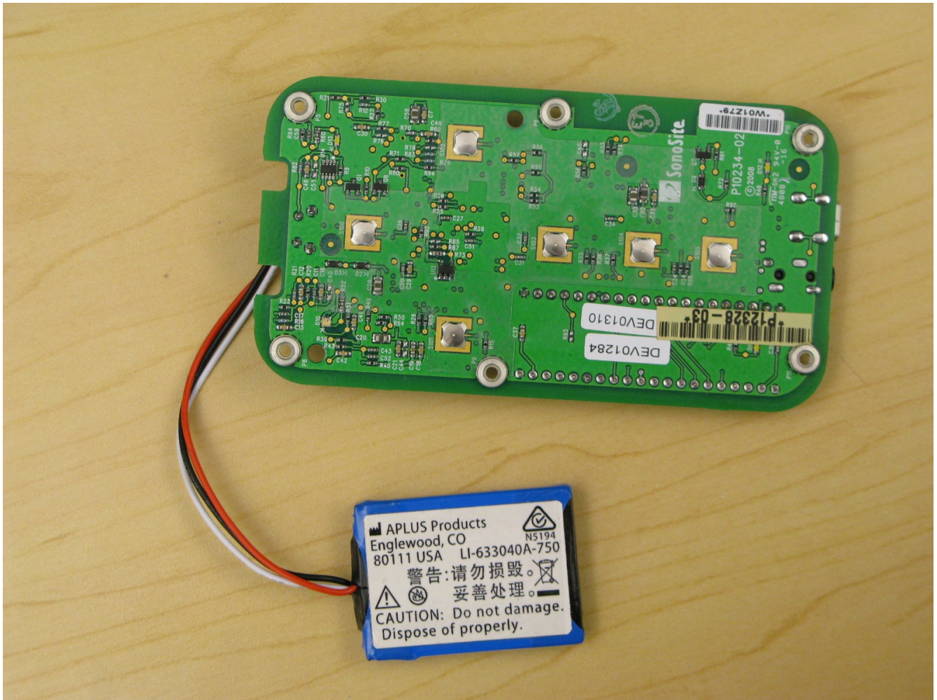
Illustration 2: Remote Control interior Bottom side
