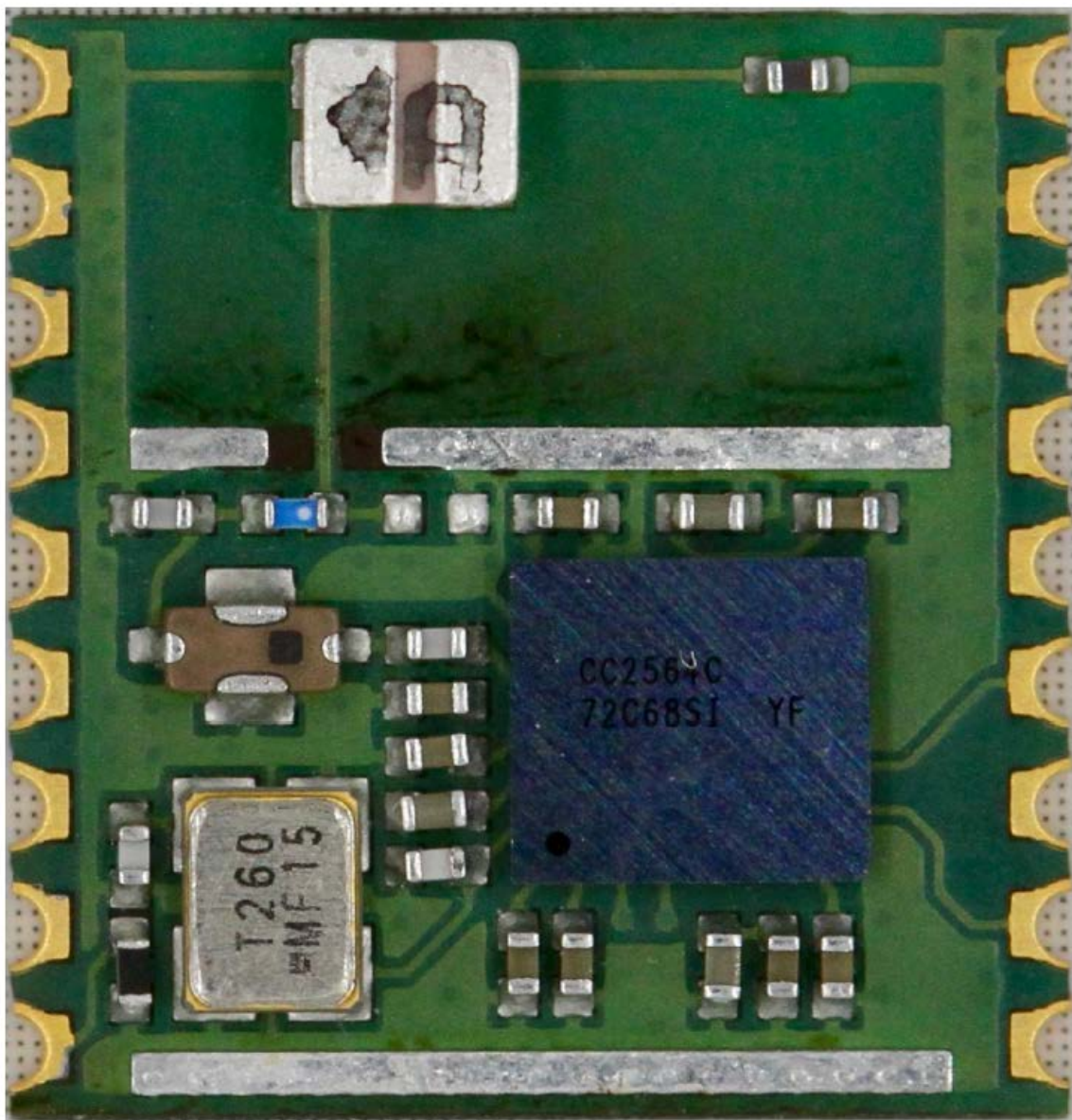
BL871E2-HI Module Top Side with shield and labelling removed
