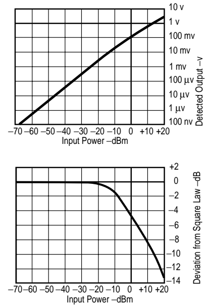
Figure 1. The diode detection characteristic ranges from square law through a transition region to linear detection.
