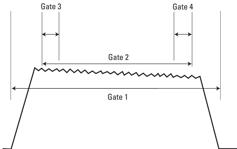
Figure 3. Powerful data configuration routines permit measurements during 4 gate times, each with 2 data “feeds” for display. Computed parameters such as peak-to-average ratio can also be displayed.
