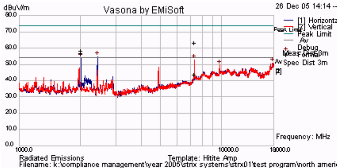
Plot 52 Radiated Emissions for Configuration # 5
