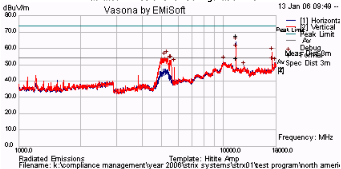
Plot 55 Radiated Emissions for Configuration # 8
