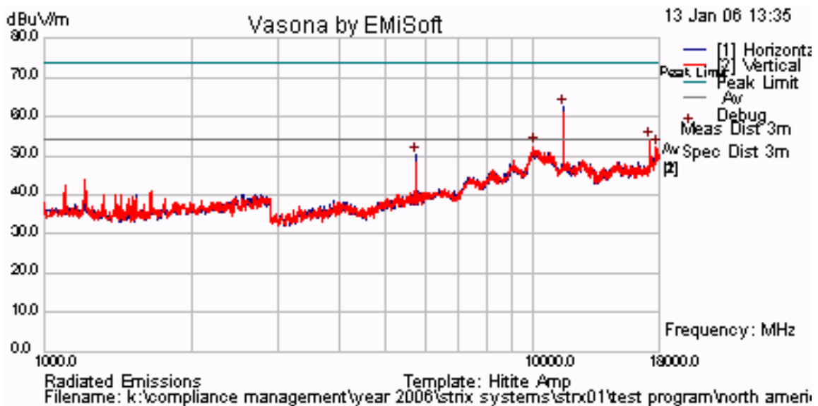
Plot 58 Radiated Emissions for Configuration # 11
