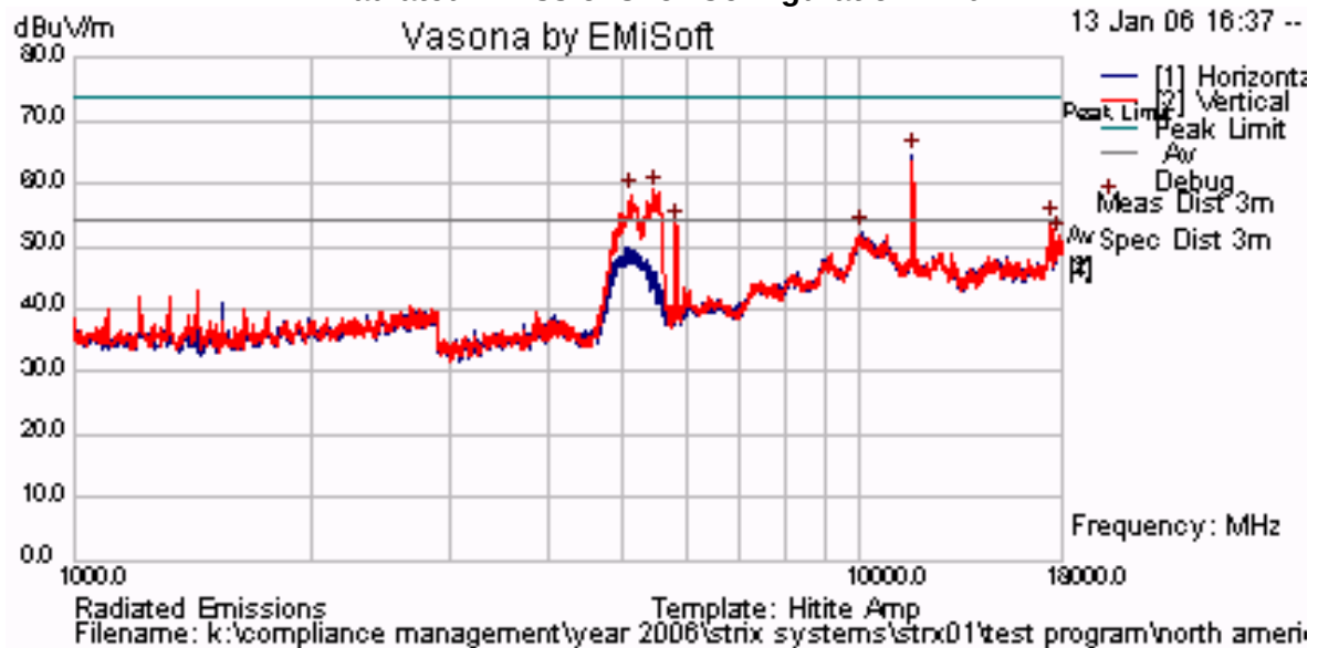
Plot 57 Radiated Emissions for Configuration # 10
