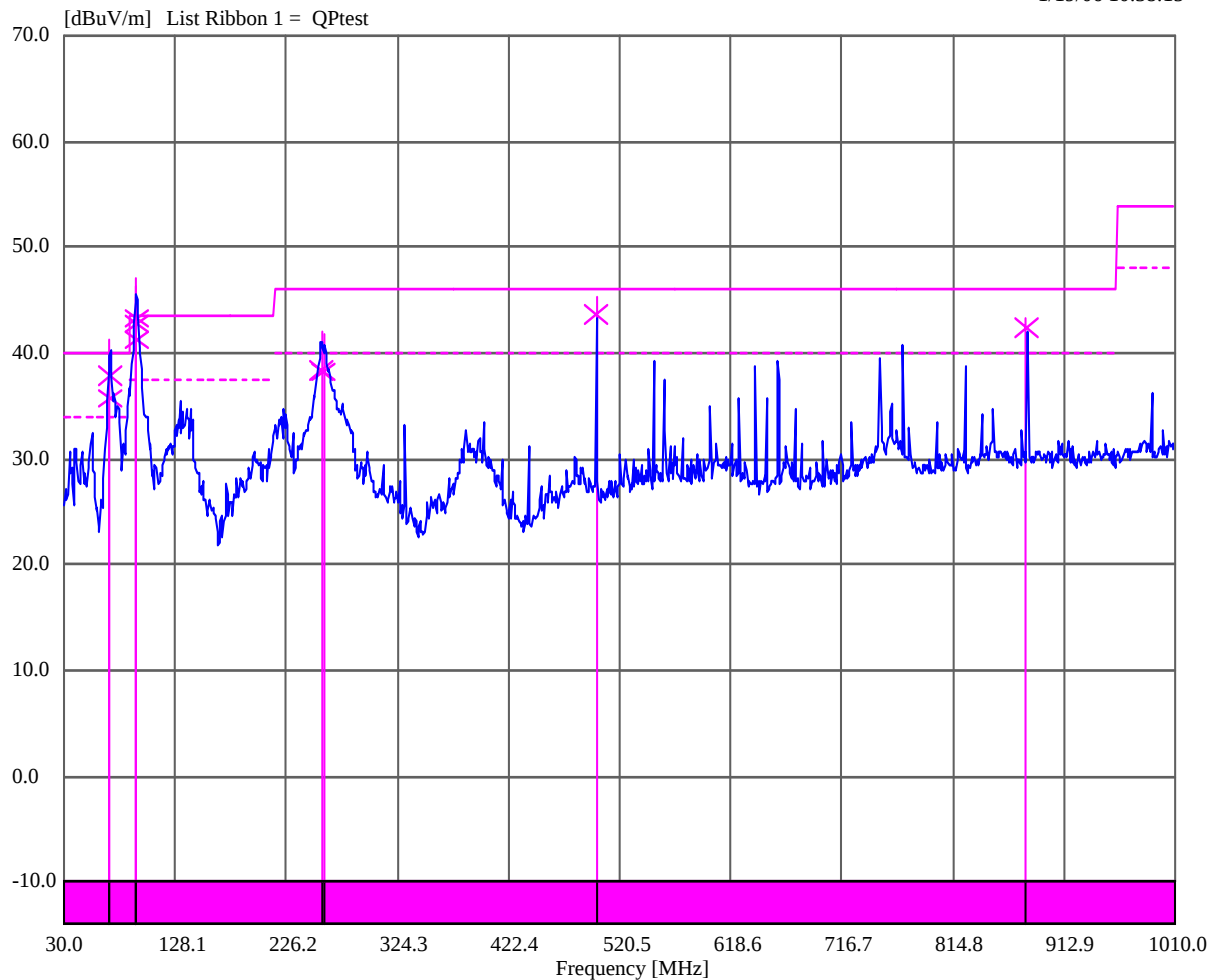
Plot 72 Radiated Spurious Emissions 30 MHz to 1 GHz
