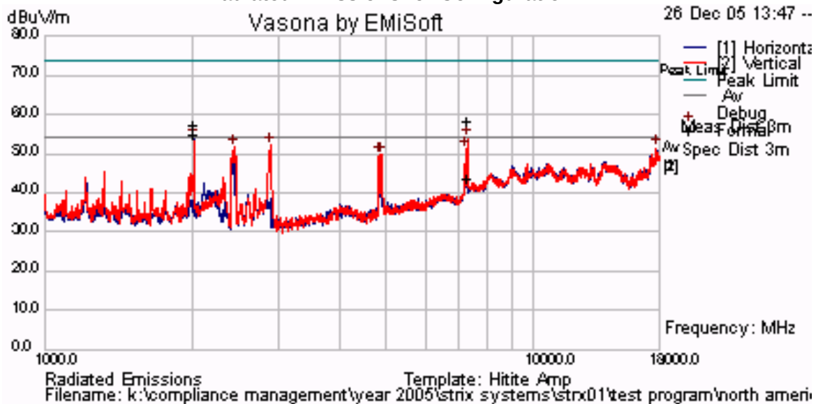
Radiated Emissions for Configuration # 4
