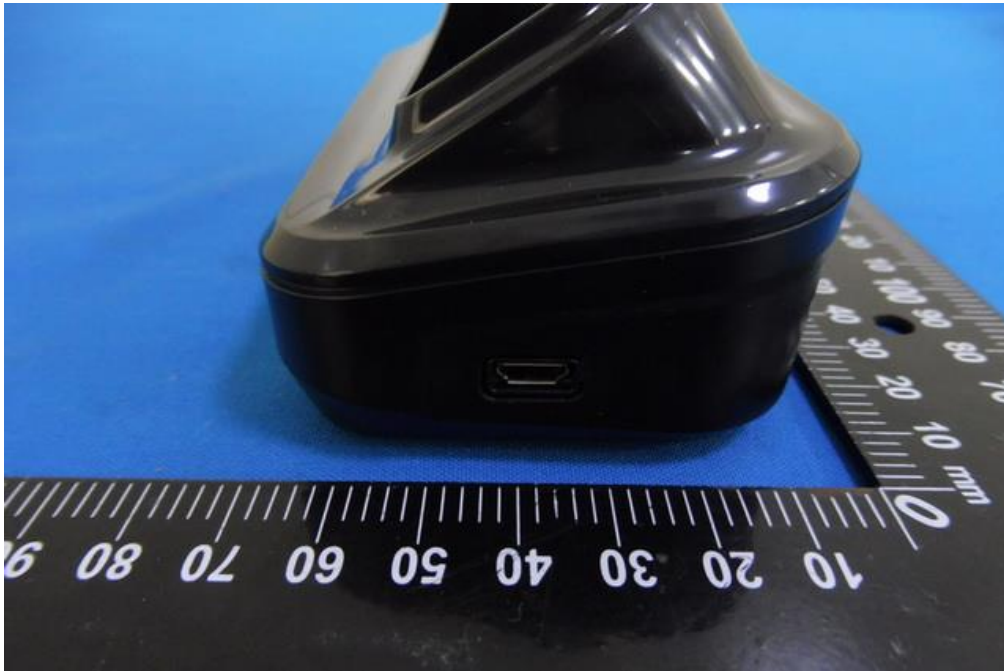
Base - Side View
