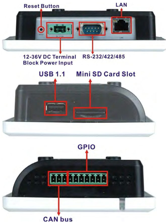
Figure 1-3: IOVU-430M Peripheral Connectors
