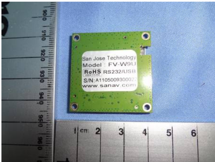
GPS module Rear View
