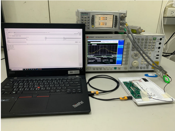
Part_15.247_WLAN_Conducted_Setup
