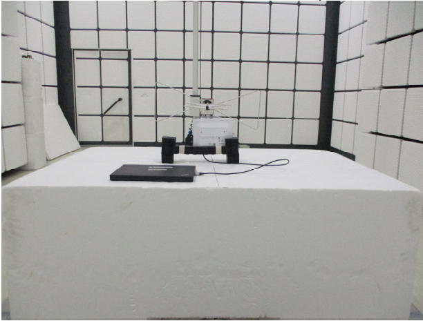
Part_15.247_WLAN_Radiated_Setup
