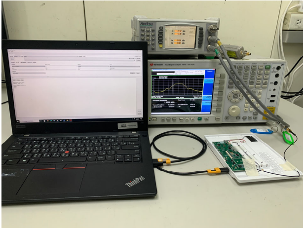
Part_15.247_WLAN_Conducted_Setup
