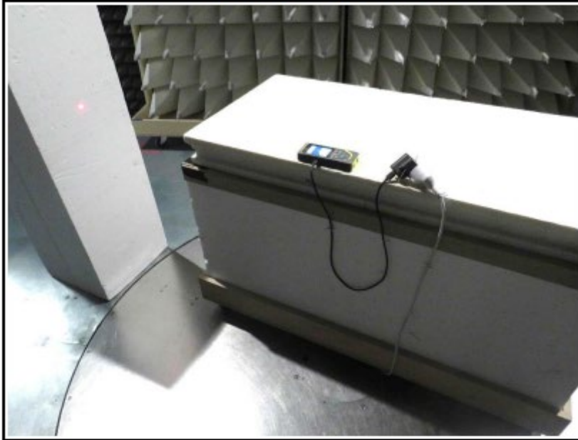
TEST SETUP – FOCUS - CONFIGURATION 2
