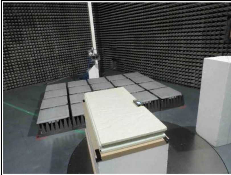
TEST SETUP – 1 GHz to 13 GHz – example CONFIGURATION 2
