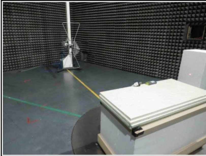
TEST SETUP – 30 MHz to 1 GHz – example CONFIGURATION 1
