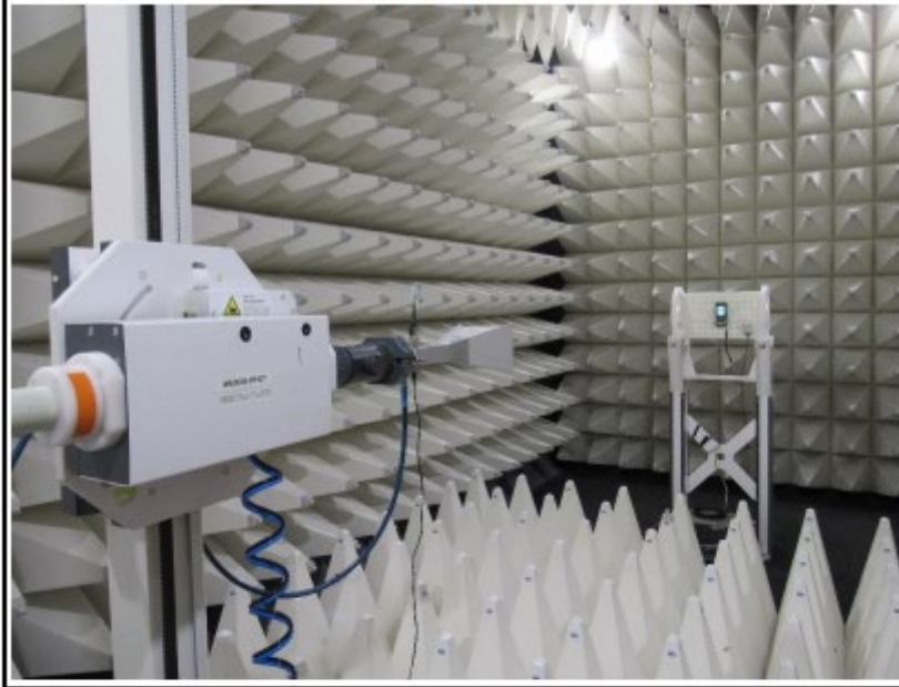
Setup for measurements above 1 GHz
