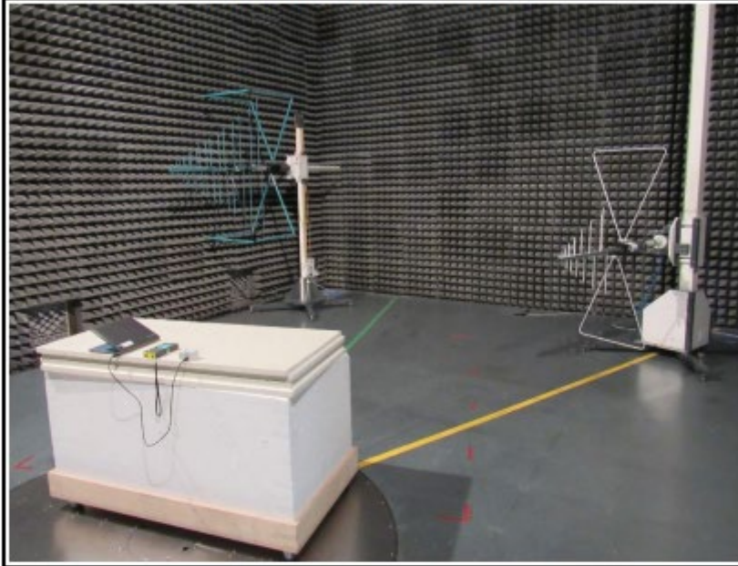
Setup for measurements below 1 GHz
