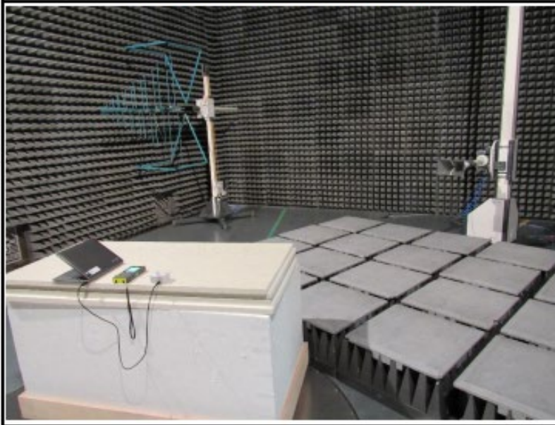
Setup for measurements above 1 GHz
