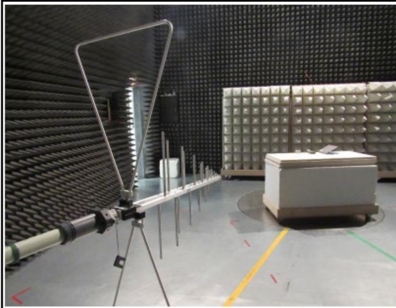
Setup for measurements below 1 GHz
