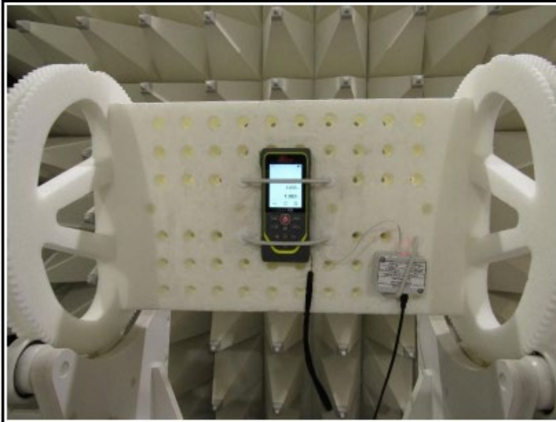
EUT Test Setup above 1 GHz
